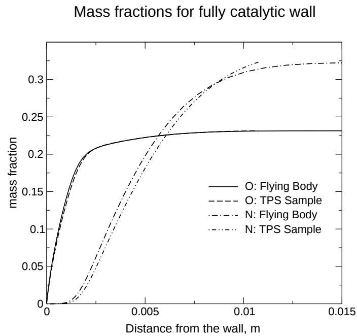
Figure 10: Case (b): O and N mass fractions for fully catalytic wall
