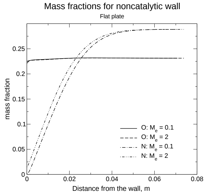
Figure 15: Flat plate O and N mass fraction at x(u_{e, M_e=0.1}/u_e) = 0.5 for noncatalytic wall
