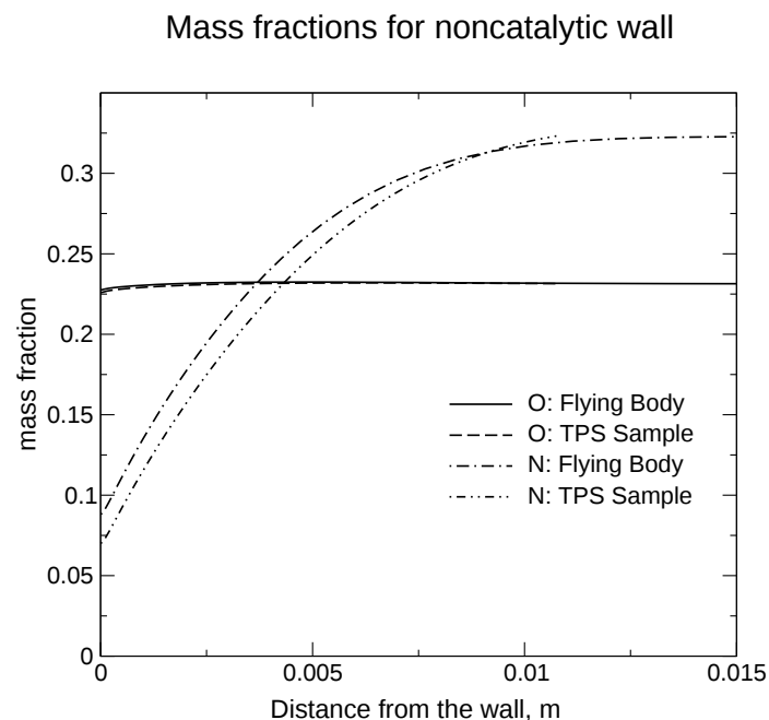
Figure 8: Case (b): O and N mass fractions for noncatalytic wall
