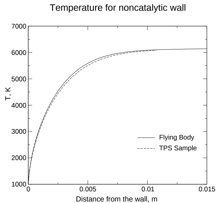
Figure 7: Case (b): temperature profile for noncatalytic wall
