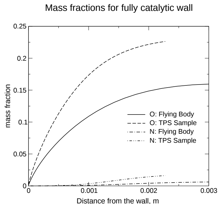
Figure 5: Case (a): O and N mass fractions for fully catalytic wall
