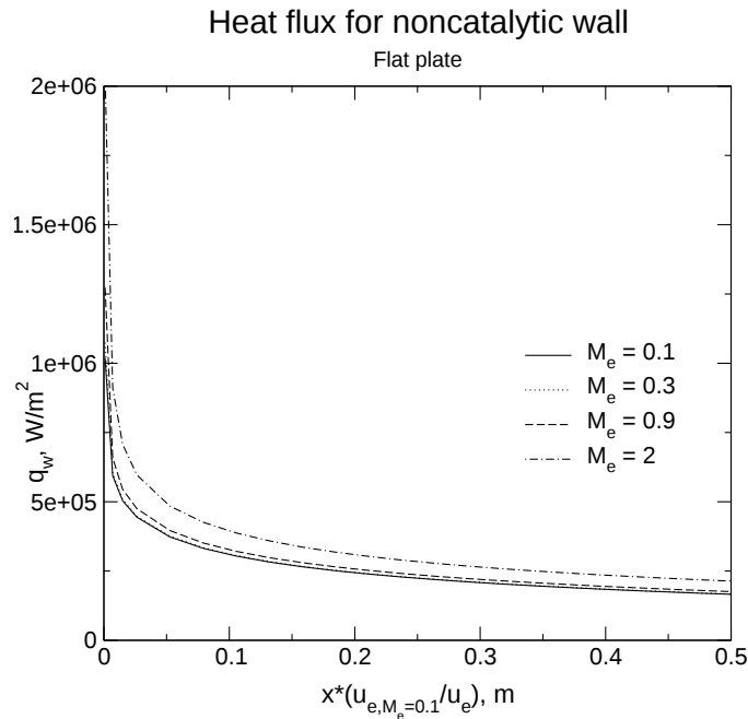
Figure 12: Flat plate heat flux for noncatalytic wall
