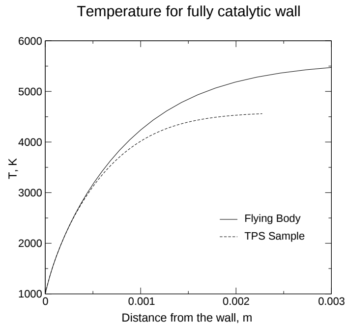
Figure 4: Case (a): temperature profile for fully catalytic wall
