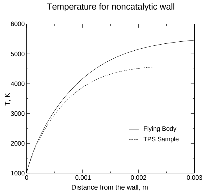
Figure 2: Case (a): temperature profile for noncatalytic wall
