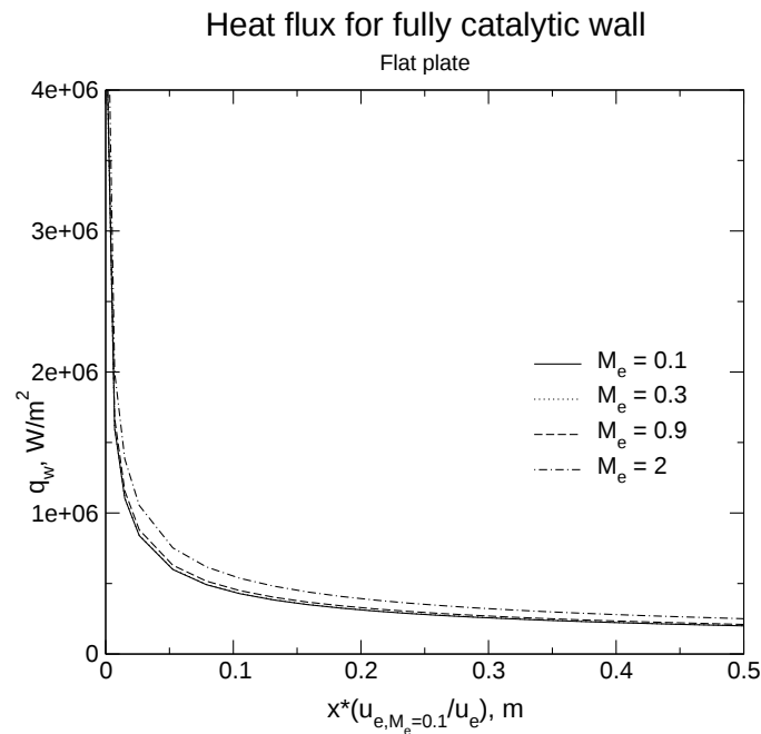
Figure 13: Flat plate heat flux for fully catalytic wall
