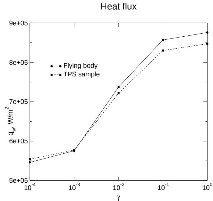
Figure 6: Case (b): stagnation point heat flux for different catalycity levels
