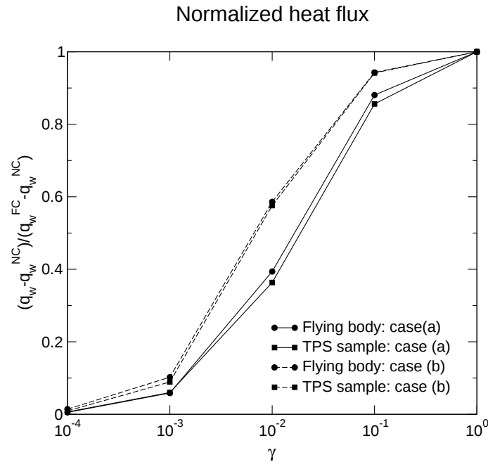
Figure 11: Stagnation point normalized heat flux for different catalycity levels
