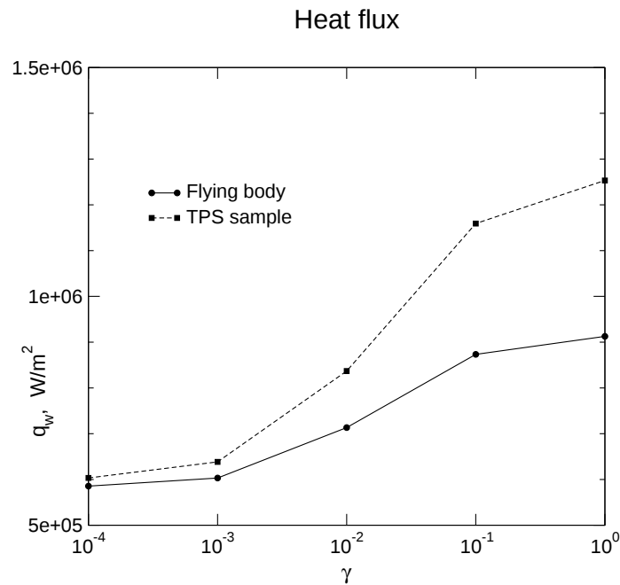
Figure 1: Case (a): stagnation point heat flux for different catalycity levels
