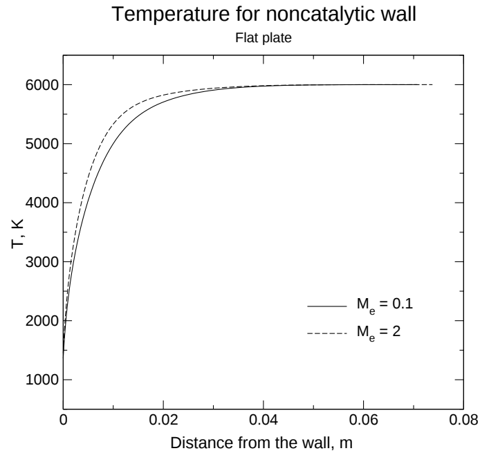
Figure 14: Flat plate temperature at x(u_{e, M_e=0.1}/u_e) = 0.5 for noncatalytic wall
