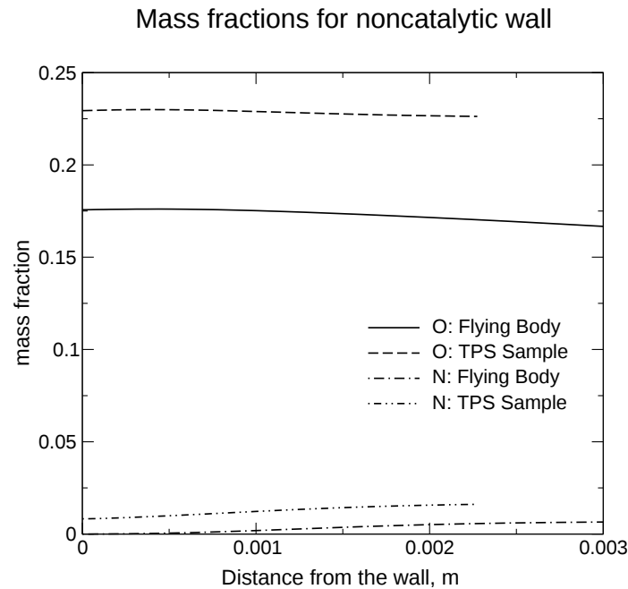
Figure 3: Case (a): O and N mass fractions for noncatalytic wall
