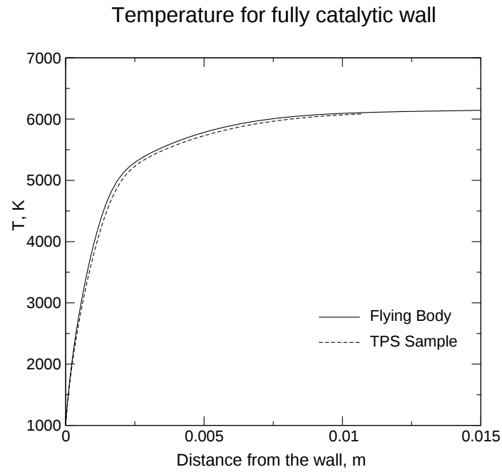
Figure 9: Case (b): temperature profile for fully catalytic wall
