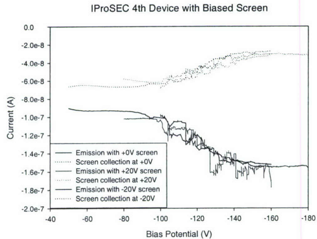
Figure 8: Fourth IProSEC Device. Screen biased at +0, -20V and +20V compared to pad bias. Note screen current in this case.
