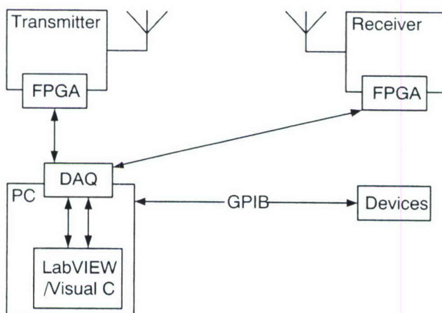
Figure 7.1: PC-based system testing architecture
