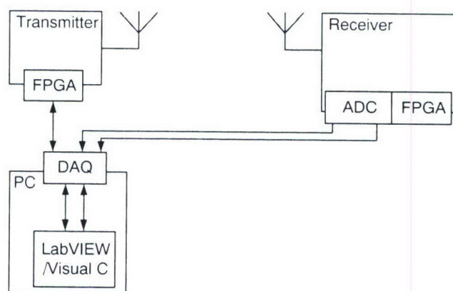
Figure 7.3: SNR test
