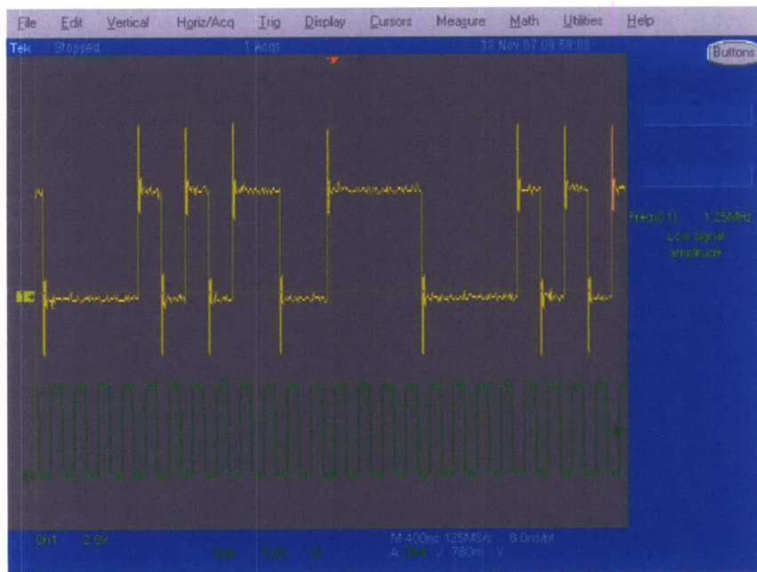
Figure 8.4: Receiver output.
