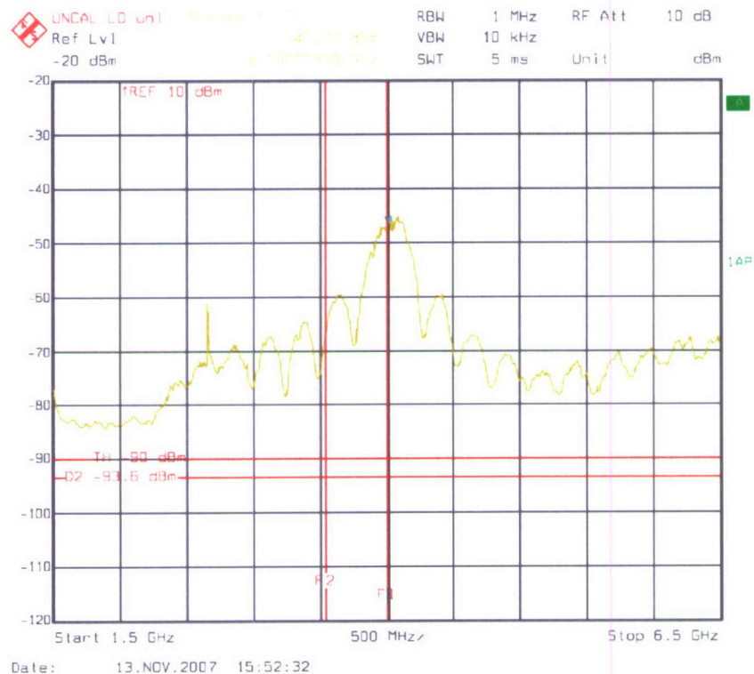
Figure 8.3: Transmitted signal spectrum.
