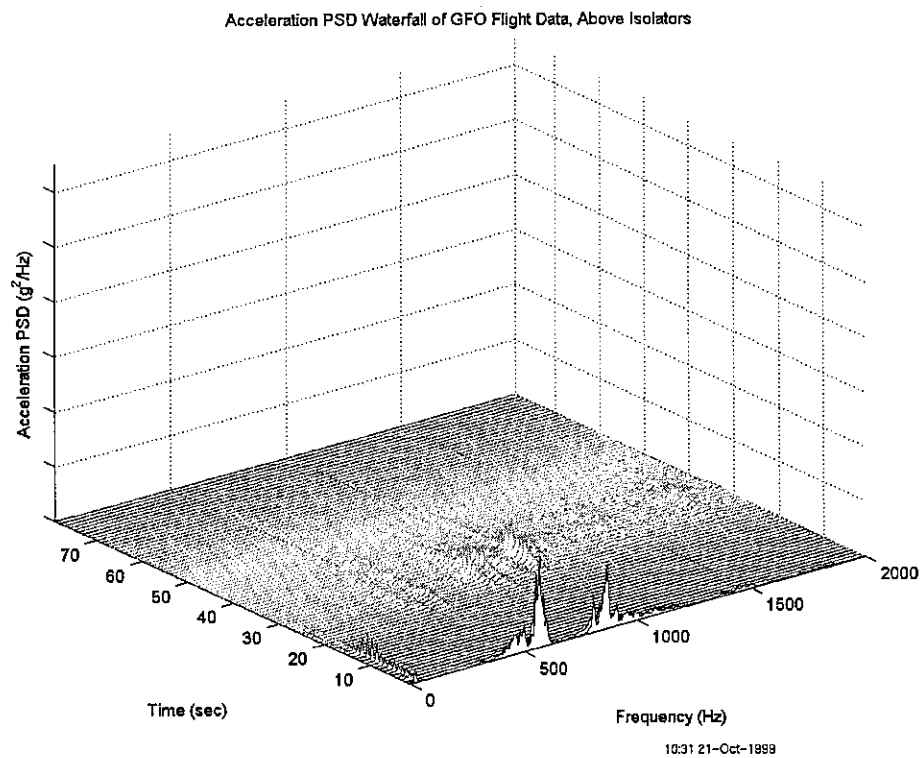
Figure 8 Waterfall PSD of GFO data - above isolators
