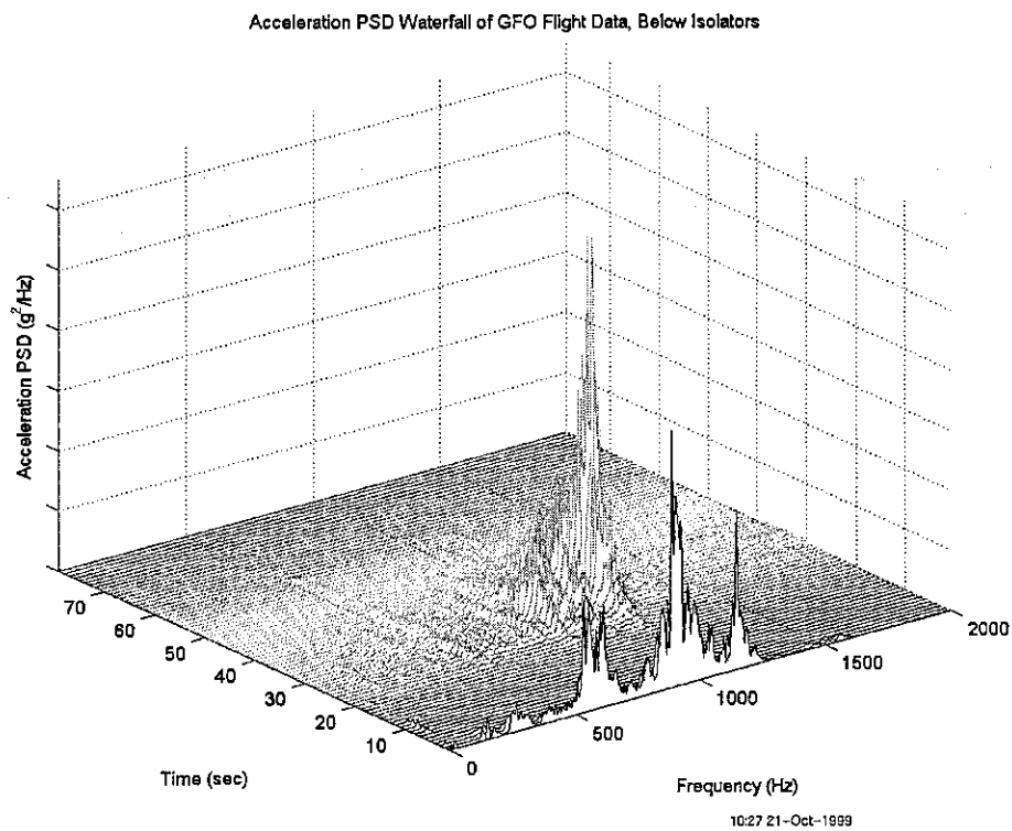
Figure 7 Waterfall PSD of GFO data - below isolators
