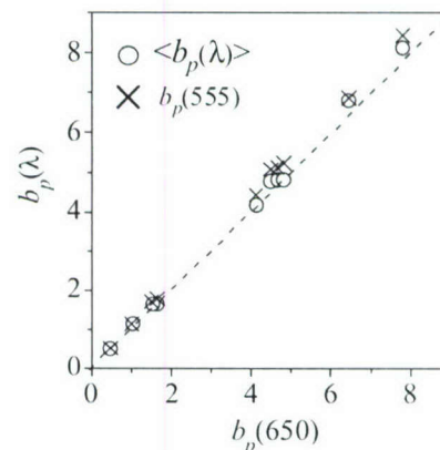
Fig. 5. Relationships between \langle b_p(\lambda) \rangle and b_p(650) , and between b_p(555) and b_p(650) , for study sites, with equivalence (1:1) line for reference.
