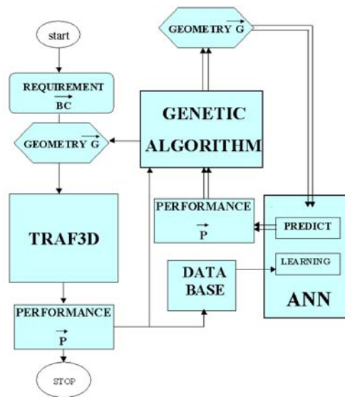
Figure 19: Flow Chart of a 2 Level Optimization Method.
