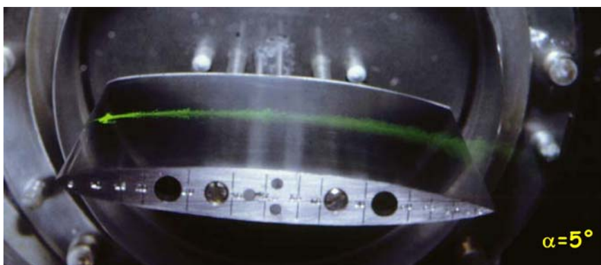
Figure 24: Laminar Separation Bubble near the Leading Edge of a Hydrofoil. The laminar separation bubble, which is a tiny dead water zone, is made visible by some spreading of dye along the span.
