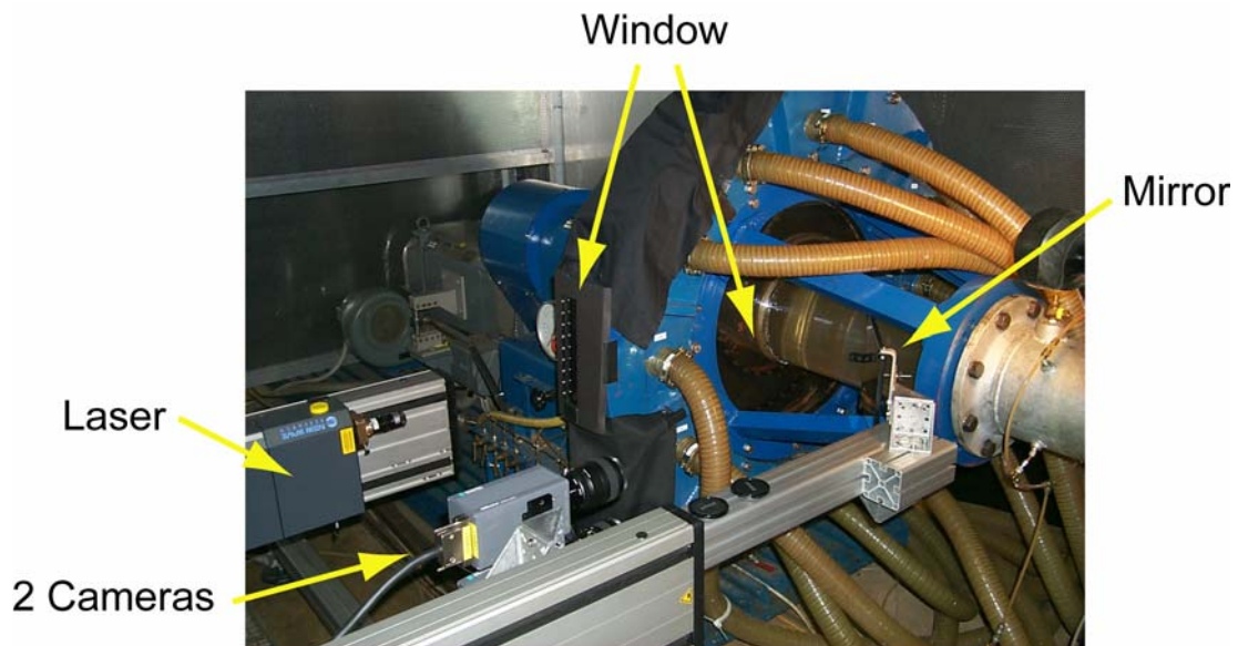
Figure 38: Picture of Test Rig for Combined PIV Measurements and Cavitation Observation.
