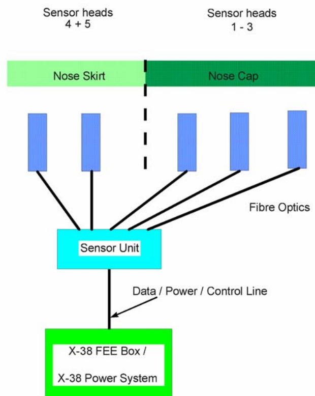
Fig. 5 Diagram of the PYREX-KAT38 system
