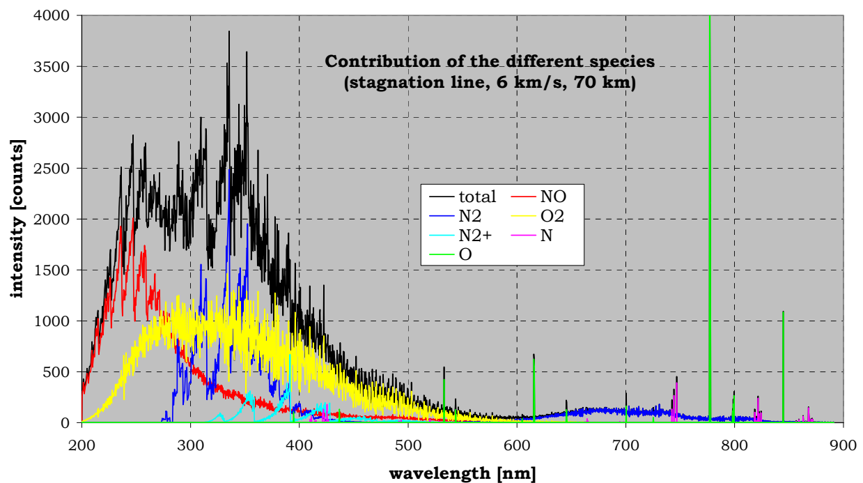
Fig. 42 Contribution of the different species to the simulated spectrometer response in counts at an altitude of 70 km for an entry velocity of 6 km/s.
