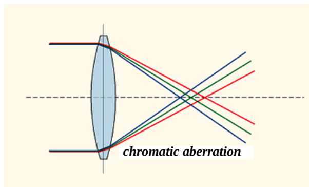
Fig. 34 Principle of chromatic aberration.
