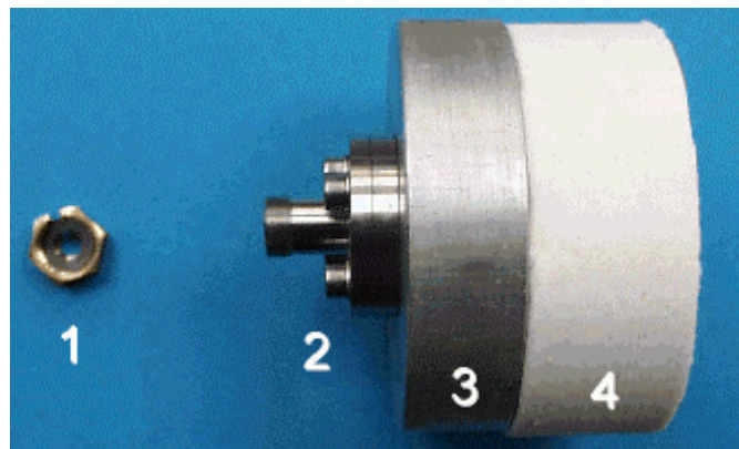
Fig. 10 Mock-up for PYREX-KAT38 PWK EM test: 1: FO fixation nut, 2: SH, 3: Al-structure (1/2 inch thickness), 4: Kapyrok TM Insulation (50 mm thickness)
