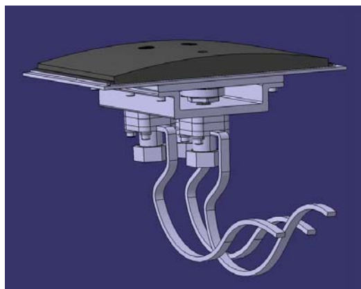
Fig. 26 Coupled sensor mount of the RESPECT sensor and two PHLUX sensor heads.
