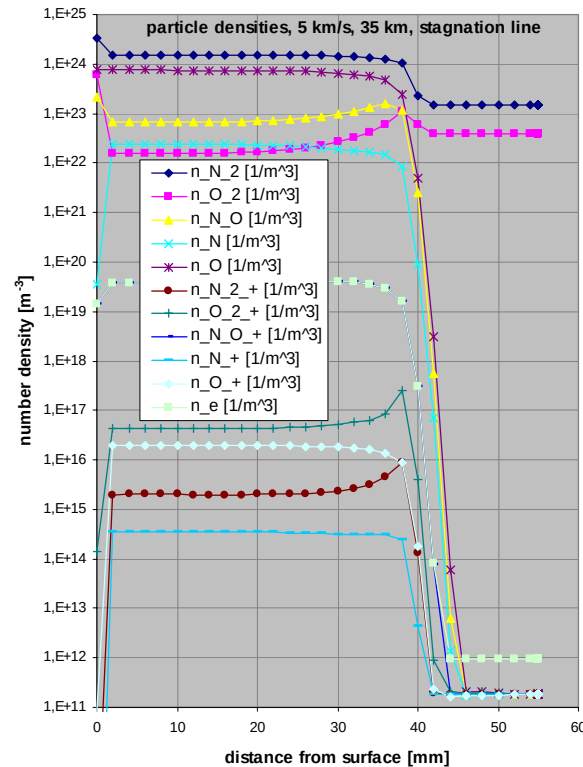
Fig. 39 Particle densities along the stagnation line for an entry velocity of 5 km/s at an altitude of 35 km.
