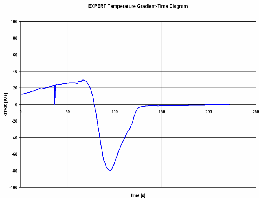
Fig. 53 Temperature gradients
