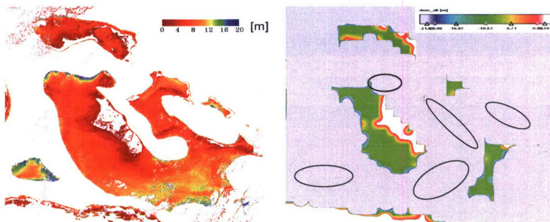
Figure 4. Bathymetry derived from MERIS (left) R_{rs}() compared with bathymetry provided with MERIS
