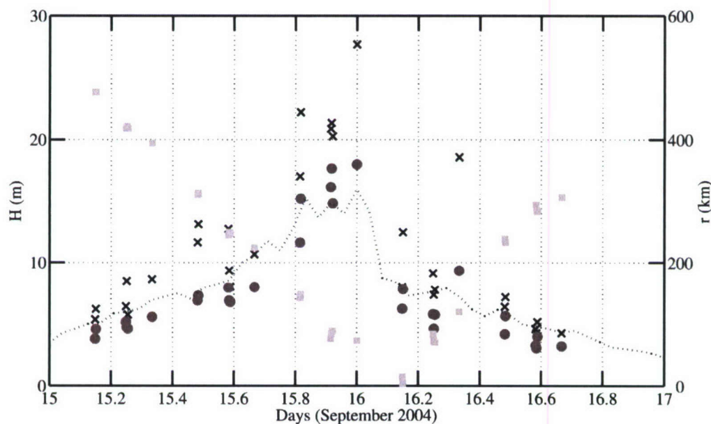
FIG. 13. Time evolution of extreme seas at the SEED moorings during the passage of Ivan. Solid circles: significant wave heights ( H_s ); crosses: maximum wave height ( H_{max} ); dotted line: significant wave height from NDBC 42040; solid squares: the distance to Ivan's center ( r ).
