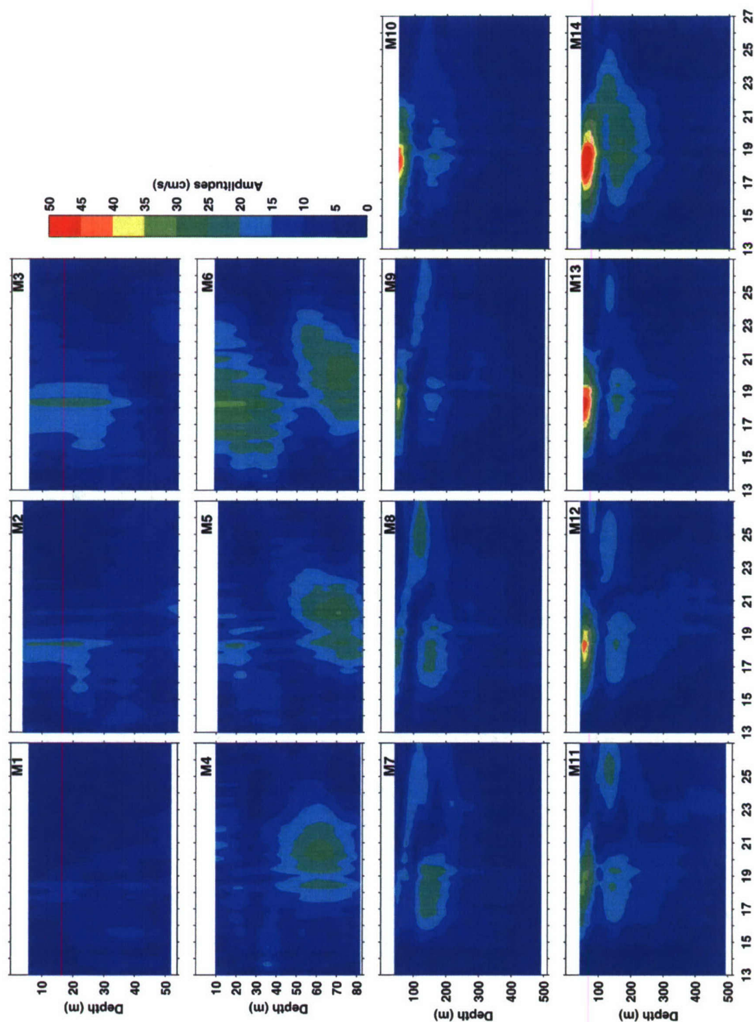
FIG. 8. Amplitude of the clockwise near-inertial motion ( \text{cm s}^{-1} ).
