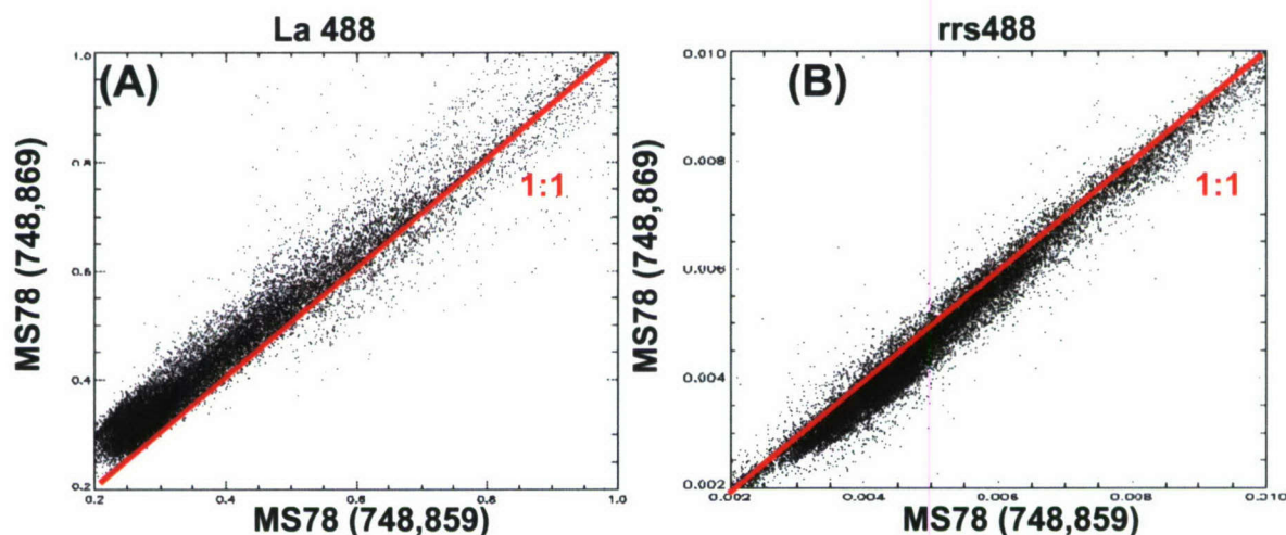
Figure 2: (A) Scatter plot showing the difference in aerosol contribution (La) at 488nm using the default 1km channel 8 (869nm) (y-axis) and the substitution of the 250m channel 2 (859nm) (x-axis) in the standard Gordon/Wang atmospheric correction. Note that there is a slight offset from the 1:1 line (red). (B) Scatter plot showing the difference in Rrs at 488nm using the default 1km channel 8 (869nm) (y-axis) and the substitution of the 250m channel 2 (859nm) (x-axis) in the standard Gordon/Wang atmospheric correction. Note that slight offset in La in Figure 2(A) does not significantly affect the resulting Rrs.
