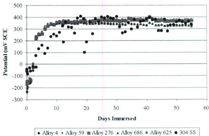
Figure 3b. OCP of Ni-Cr-Mo alloys and 304SS during 60-day exposure at Delaware Bay, showing corrosion potential ennoblement approaching 300 mV in the first 7 days. (Martin et al., 2007)
