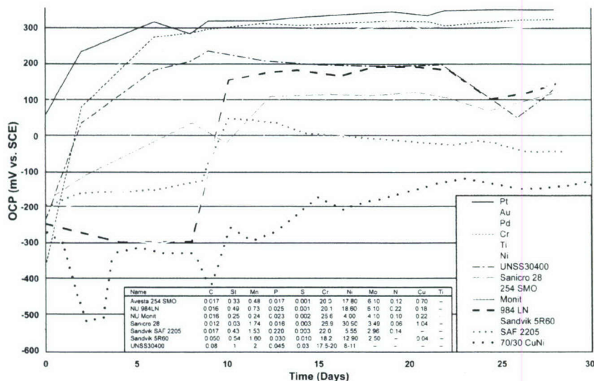
Figure 2. Composite of OPC vs. time data for materials exposed in natural seawater. Data were taken from Ito et al., 2002; Johnsen & Bardal, 1985; de Mele, 1992. Prepared by Jason S. Lee, Na Research Laboratory
