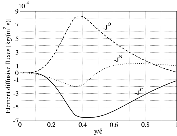
Figure 4: Elemental diffusive fluxes ( -\mathcal{J}_e ).
