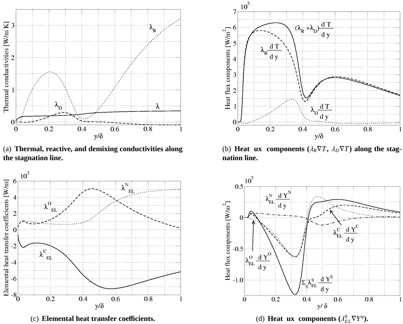
Figure 7: Heat flux components, thermal conductivities, and elemental heat transfer coefficients.
