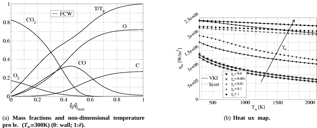
Figure 18: Stagnation line solution for the higher enthalpy case (Park bulk chemistry model) [ h_\delta=39\text{MJ/kg} ].
