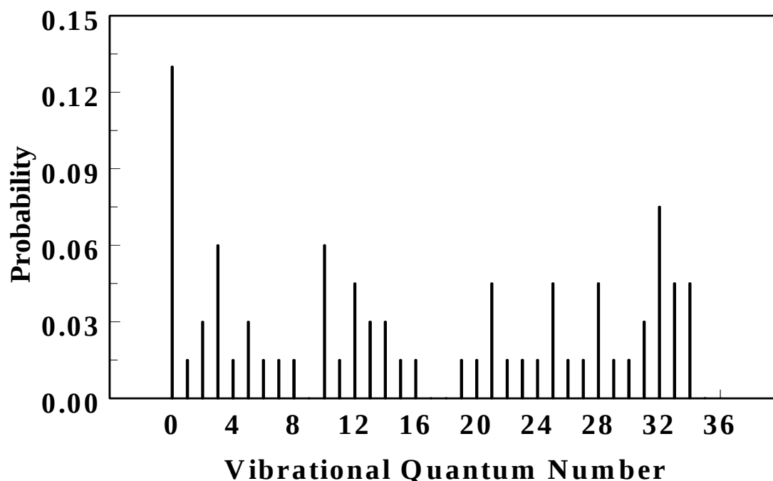
Fig.14: A typical vibrational distribution of the O_2 molecules formed after atom recombination over \beta -cristobalite at E_{kin} = 0.003\text{eV} and T_s = 1000\text{K} .
