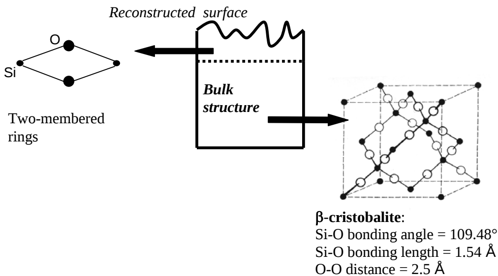
Fig. 6: A reconstructed surface is depicted.
