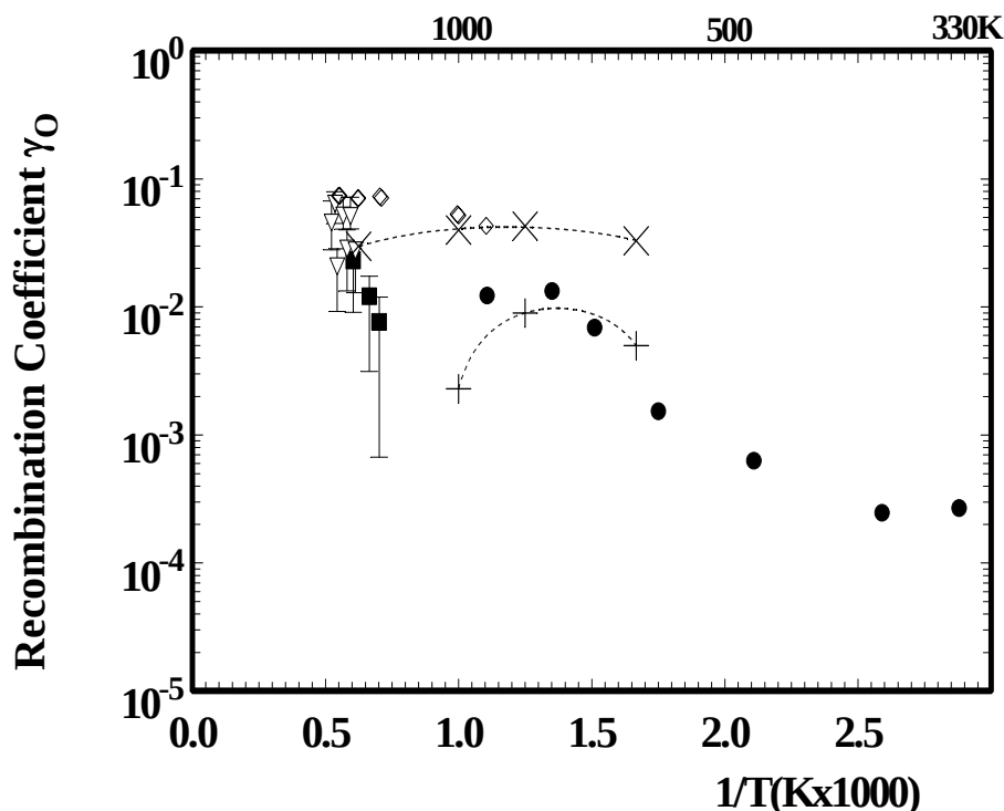
Fig. 10 : The semiclassical recombination coefficient \gamma for the E-R (X ) and the L-H (+) recombination reaction [21] is reported together with the experimental data ( ■ Scott (silica-based materials) Ref. [3]; • Greaves et al. (silica) Ref. [4] ; Berkut et al. (silica-based materials) Ref. [2] ; ◇ Balat et al. ( \beta -cristobalite) Ref. [31] ).
