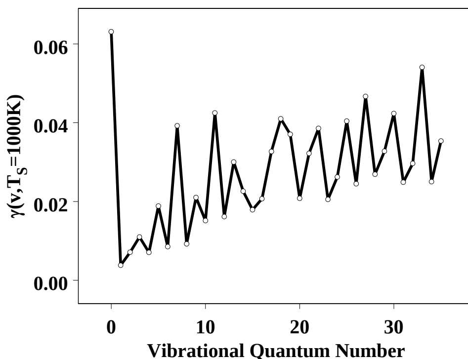
Fig.15: The vibrational spectral distribution of the recombination coefficient \gamma for O_2(v) formed in the reaction: O + O_{ad} \cdot \text{silica} \rightarrow O_2(v,j) + \text{silica} is reported as a function of the vibrational quantum number v . T_s=1000K .
