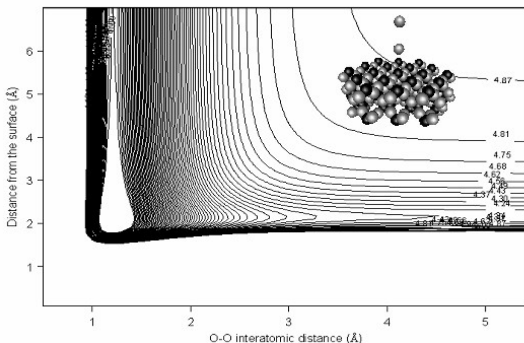
Fig. 5: Two-dimensional interaction potential for O 2 interacting in the perpendicular orientation on top of a Si atom of a \beta -quartz surface. The potential (in eV) is plotted as a function of the O-O internuclear distance and the distance of the closest O atom to the surface.
