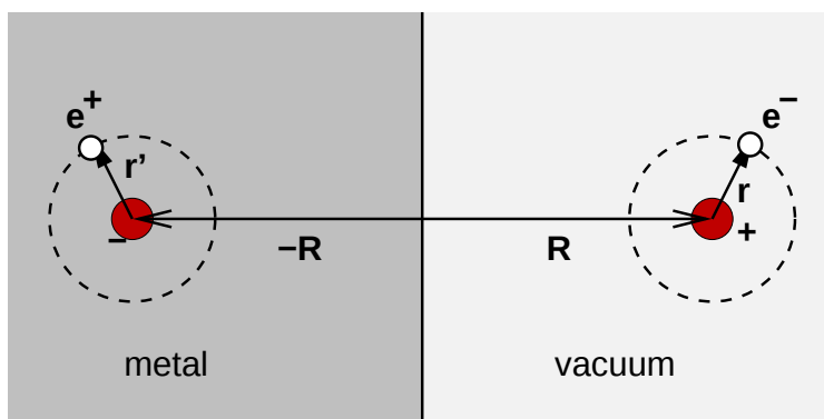
Figure 9: Van der Waals interaction: schematic illustration of a hydrogen atom in front of a perfect conductor interacting with its image charges.
