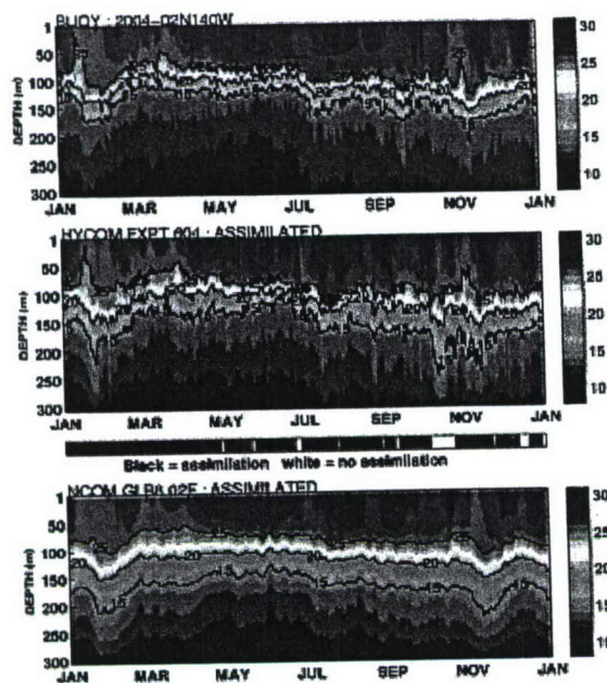
Figure 2. Subsurface temperature at 140W,2N down to 300m in 2004 from a) the TAO buoy, b) hindcast HYCOM and c) operational NCOM. The black and white bar indicates when TAO profiles were assimilated into HYCOM.
