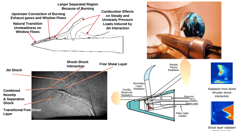
Figure 49: Aerothermal and Radiation Studies of Divert Thruster Performance with Duplicated Vehicle and Solid Propellant Rocket Motor
