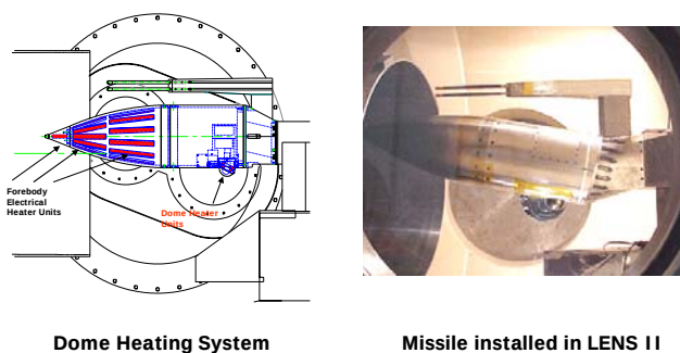
Dome Heating System
