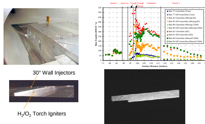
Figure 79: AFOSR Studies of Mach 7 Hydrocarbon Engine
