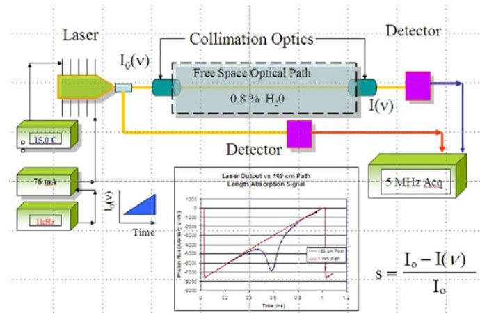
Figure 87: Schematic Diagram of Laser Diode System for Water Vapor and Temperature Measurements in Scramjet Engines
