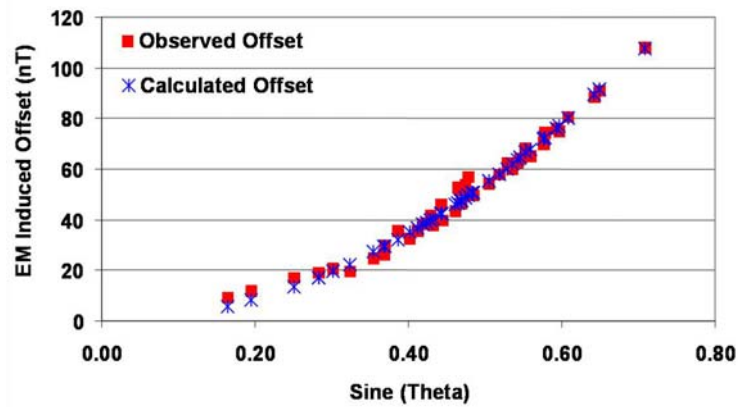
Figure 5. Magnetic offsets vs. angle between primary field and geomagnetic field.
