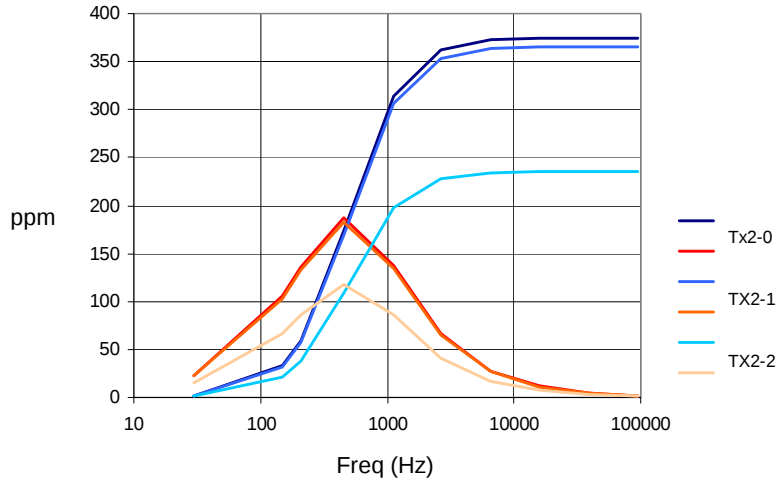
Figure 15. Measured Q-coil responses at three receiver locations.
