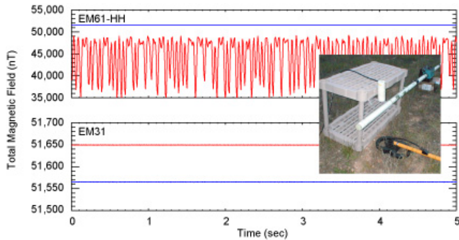
Figure 1. TMF data with (red) and without (blue) EMI sensors operating nearby.
