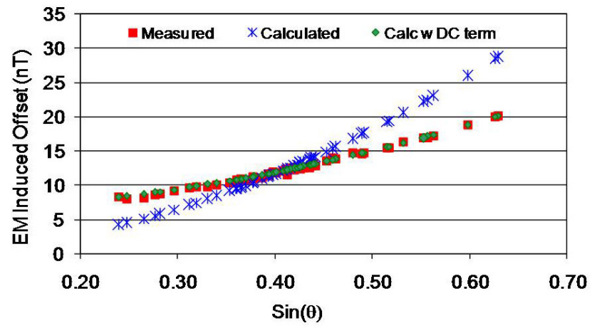
Figure 7. EMI induced offsets with DC correction factor for GEM-3.
