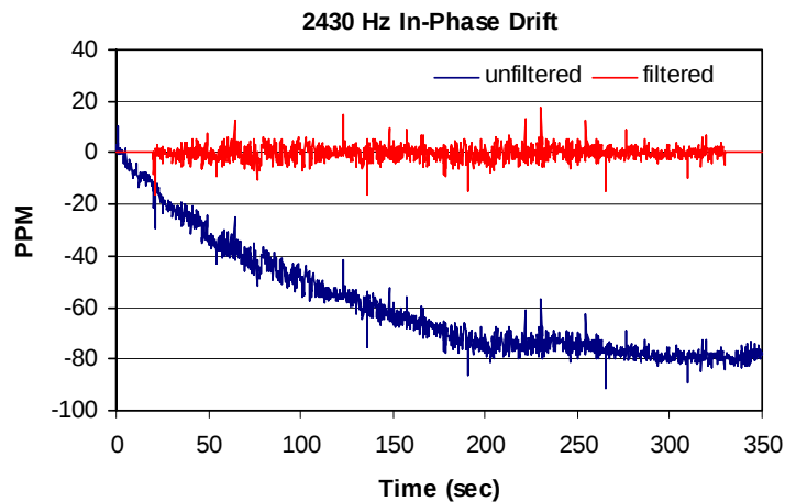
Figure 16. Warmup drift for the GEM-3 array at the Tx2-2 sensor location.
