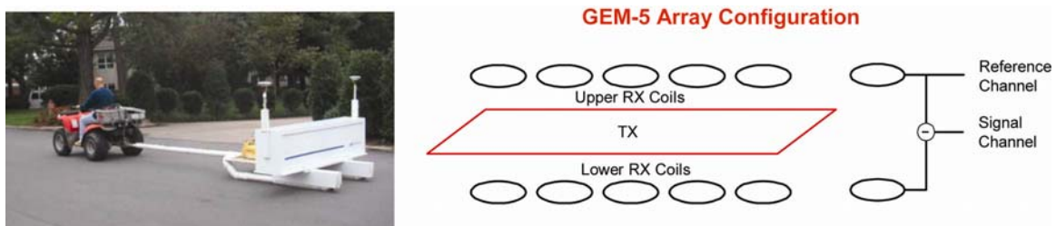
Figure 10. GEM-5 coaxial array configuration.
