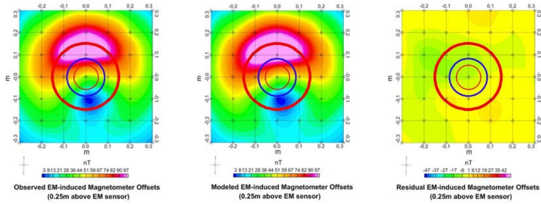
Figure 4. Observed, modeled, and residual EM-induced errors in the measured magnetic data. The EM73 transmit coil positions are shown in red. The asymmetry in the residual error plot occurs near the physical location of the transmit driver interface connection.
