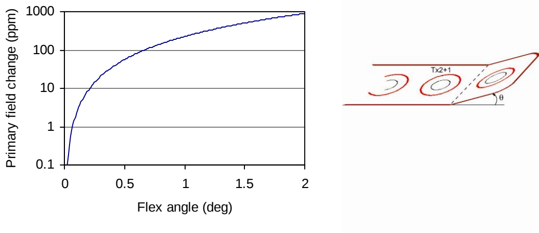
Figure 17. Effect of array flexure on primary field cancellation.
