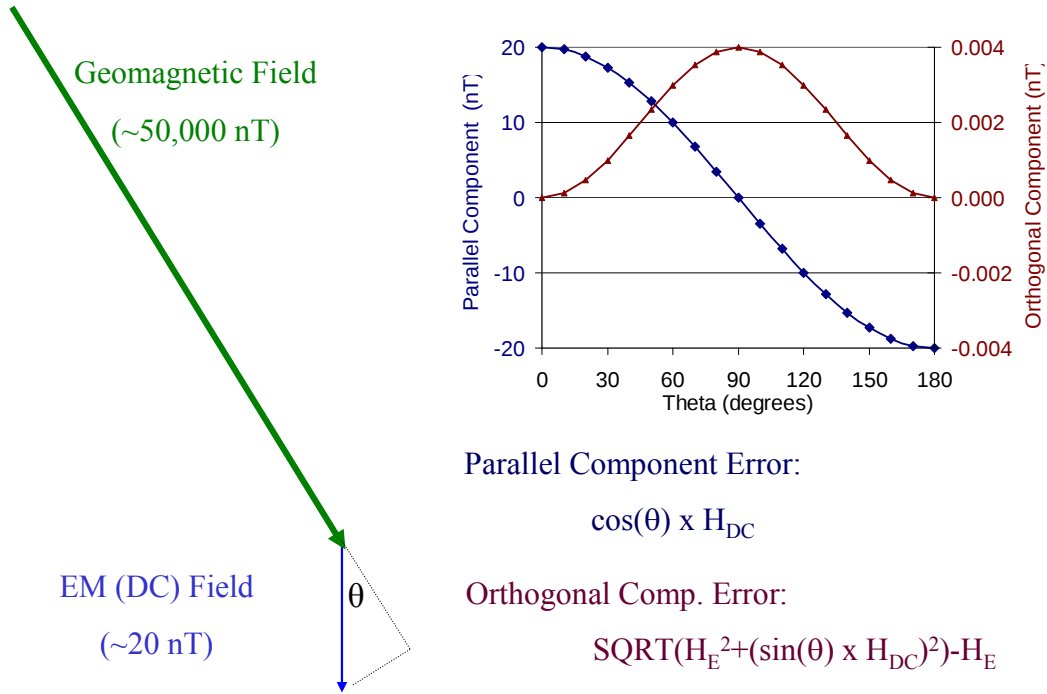
Figure 6. Induced heading errors for DC field components.
