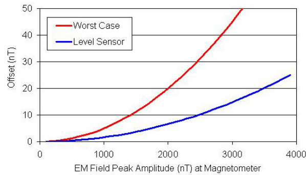
Figure 3. Nominal and worst case EM induced heading errors as a function of primary field strength at the magnetometer.
