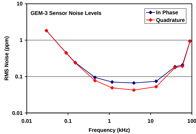
Figure 8. Sensor noise level vs. frequency for standard GEM-3.
