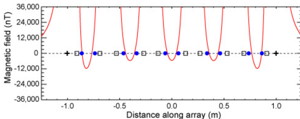
Figure 18. Magnetic field along array axis at peak transmit current (2.67 kHz).
