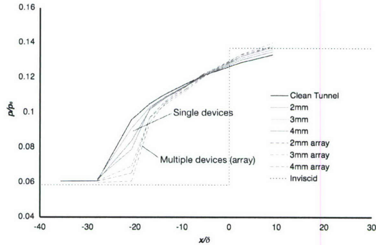
Figure 13. Centre-line surface pressure distribution through interaction with and without control.
