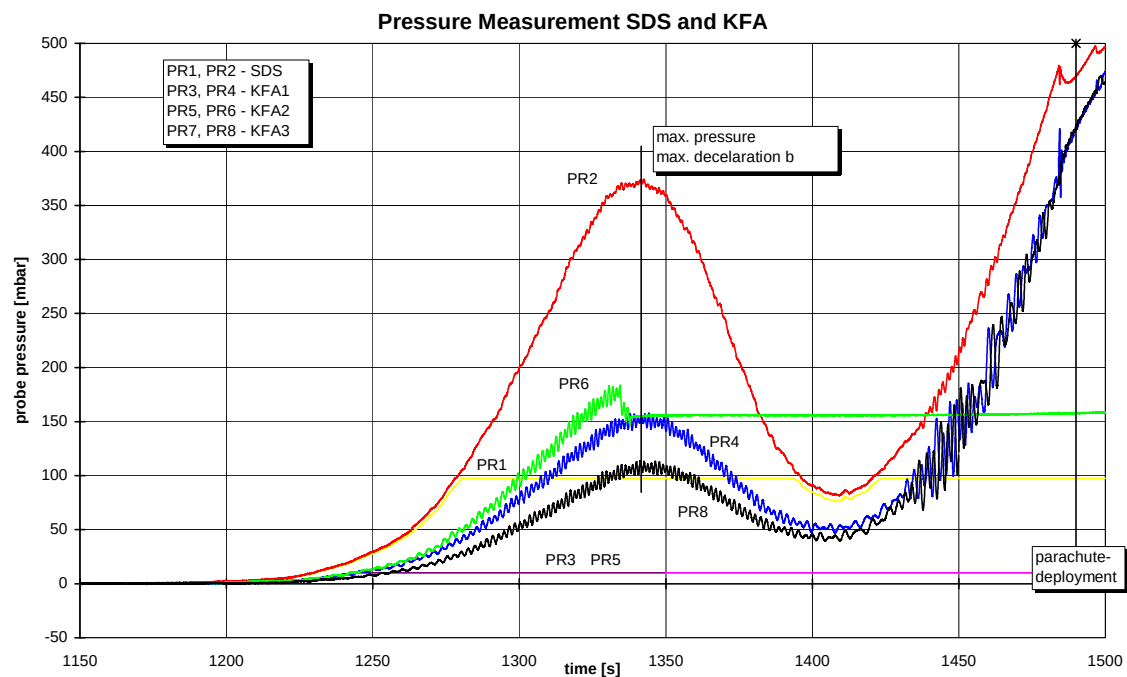
Fig. 21 Recorded RAFLEX pressure during MIRKA re-entry
