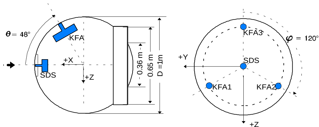
Fig. 13 Geometry of MIRKA Capsule with sensor locations
