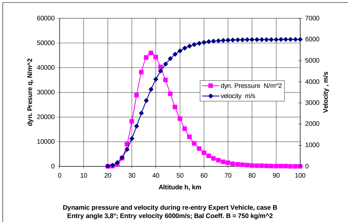
Fig. 8 Dynamic pressure and velocity EXPERT Case B, Sensor length 30 mm; B = 750 kg/m 2 , entry angle = 3,8°
