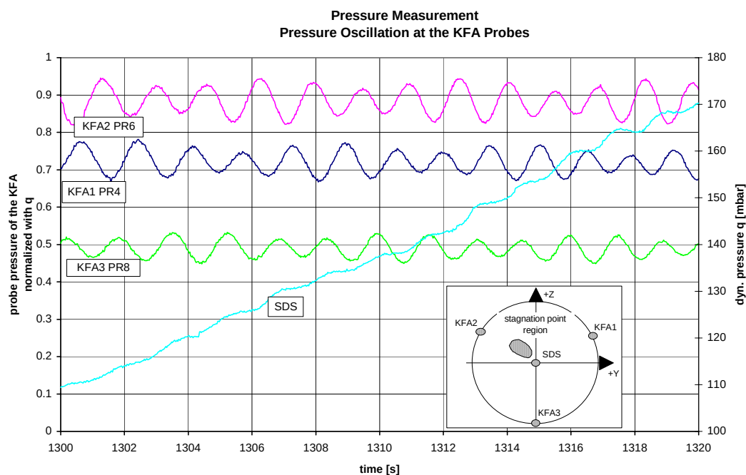
Fig. 22 Evaluated RAFLEX pressure during 20 s time period ( 1300-1320s
