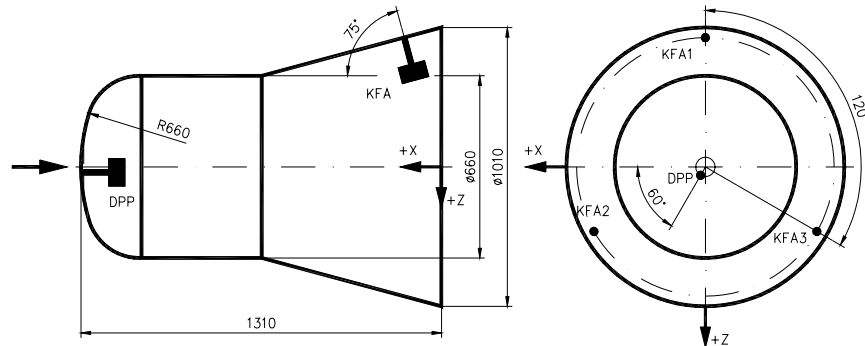
Fig 12 Raflex installation on Express Capsule
