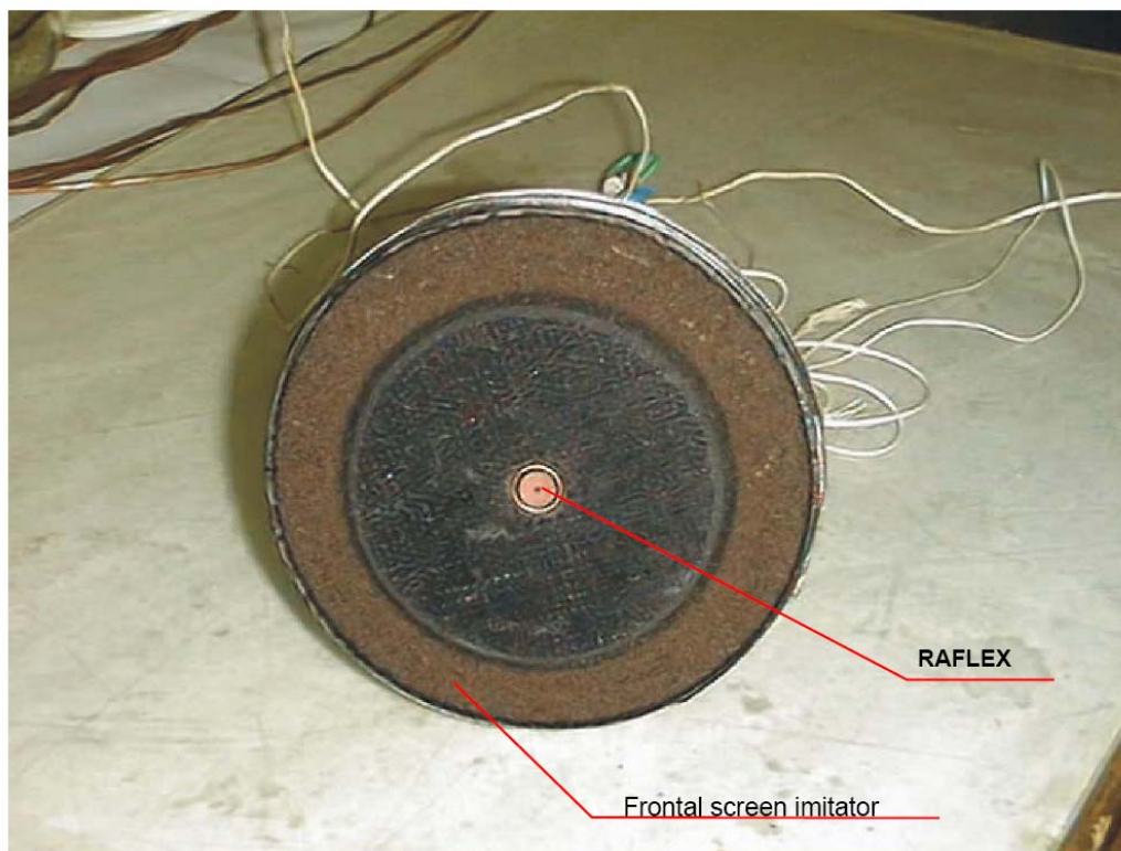
Fig. 19 IRDT2 RAFLEX III stagnation point probe after the heat load testing
