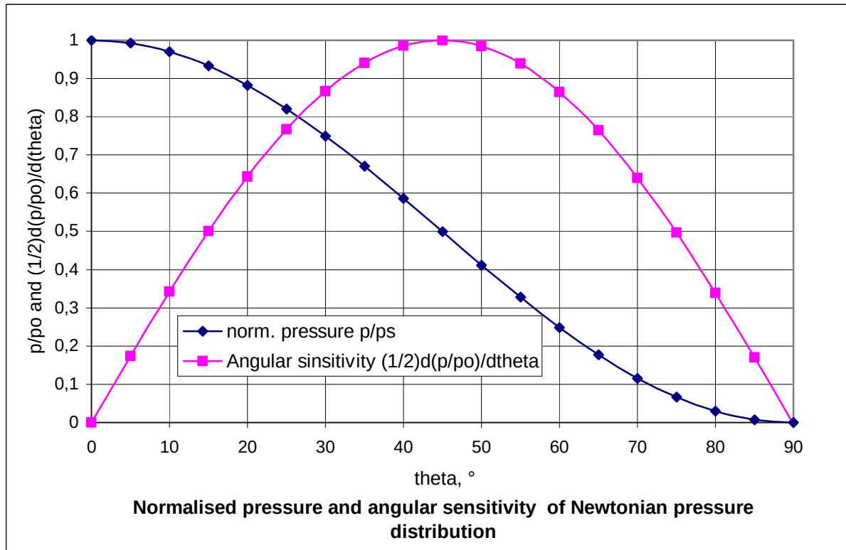
Fig. 7 Normalized Newtonian pressure distribution and angular sensitivity for one pressure tap
