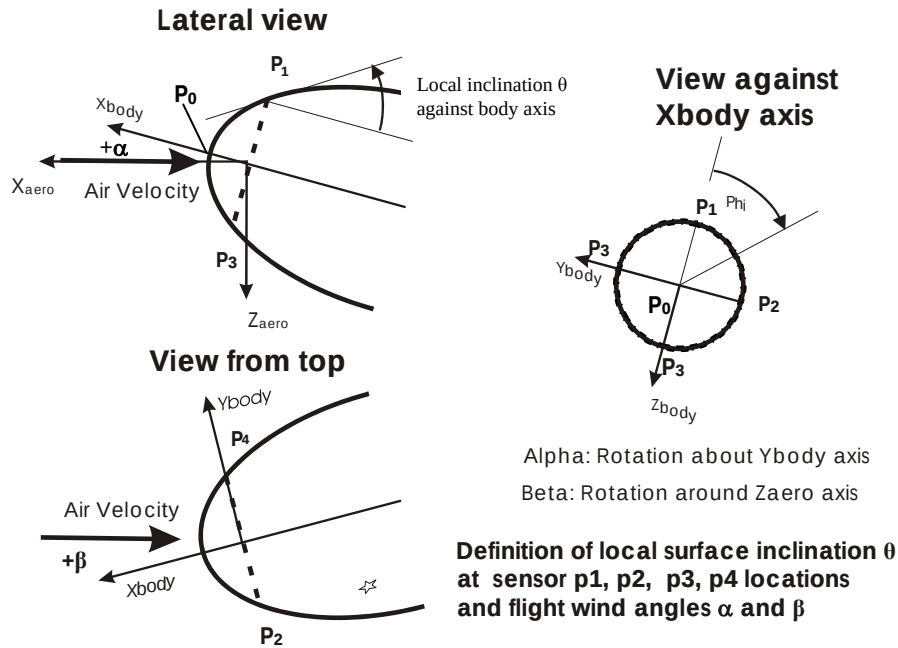
Fig 4 Definition of local surface inclination and flight wind angles
