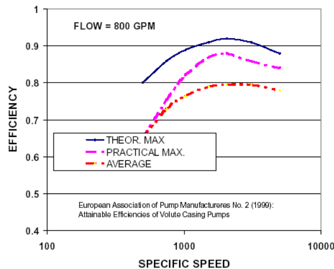
Figure 7: Theoretical Attainable Maximum Efficiency for a Volute Casing Single Stage Pumps.
