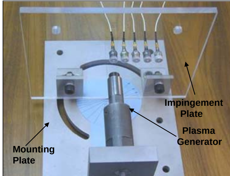
Figure 1. Experimental setup.
