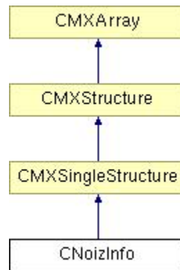
Figure 14. Inheritance diagram for CNoizInfo .
