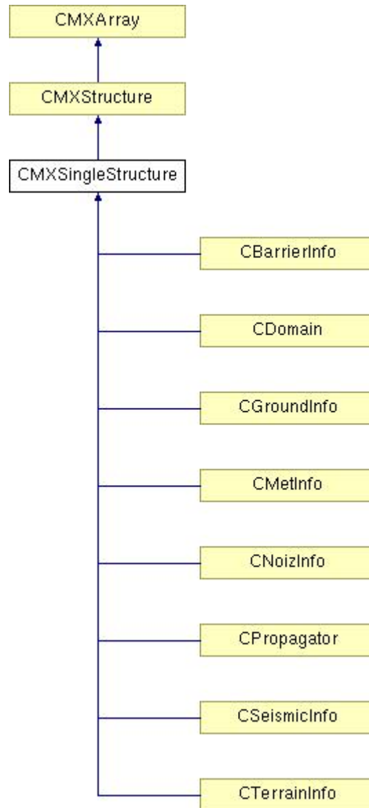
Figure 9. Inheritance diagram for CMXSingleStructure .
