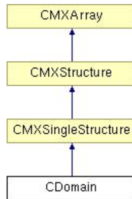
Figure 11. Inheritance diagram for CDomain .
