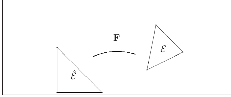
Figure 1. reference element, \hat{\mathcal{E}} and mapping \mathbf{F} : \hat{\mathcal{E}} \rightarrow \mathcal{E}
