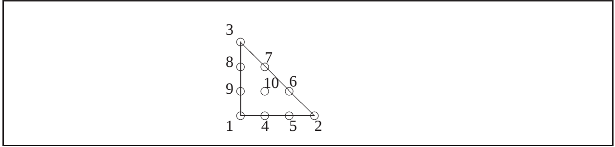
Figure 2. Standard Lagrangian nodal locations on reference element \hat{\mathcal{E}} for P^3 (triangles)
