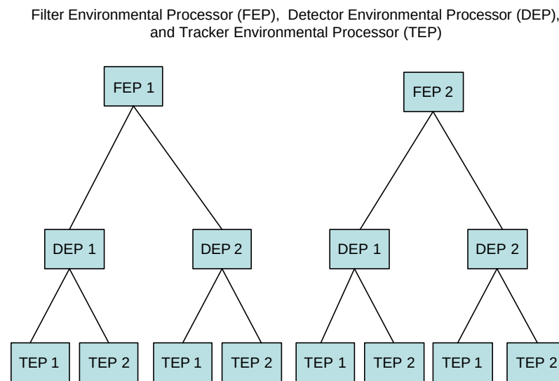
Figure 3. Parallel Algorithms
