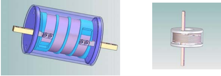
Figure5: Helical and Co-axial Inductors
