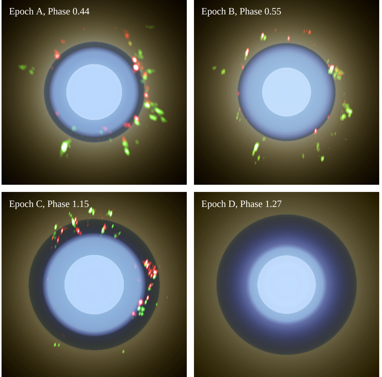
Fig. 7. The (red) \nu = 2 , J = 1-0 (42.8 GHz) and (green) \nu = 1 , J = 1-0 (43.1 GHz) maser images overlaid onto pseudo-color representations of the infrared intensity. The continuum photosphere (in fact mostly hidden behind the molecular atmosphere in the N -band) is enhanced to a light blue color. The darker blue shades represent our model intensity profile as in panels (e) of Figs. 2–5, and the green shades represent the location of the \text{Al}_2\text{O}_3 dust shell on top of the low-intensity extended wings of the molecular atmosphere. The true location of the star relative to the maser images is unknown. Here, we assume that the center of the star coincides with the center of the maser spot distribution. Synthesized beam sizes for epoch A are 0.59 \times 0.40 mas and 0.60 \times 0.37 mas for the \nu = 1 and \nu = 2 transitions, respectively. For epoch B these sizes are 0.52 \times 0.21 mas and 0.51 \times 0.20 mas, and for epoch C 0.46 \times 0.16 mas and 0.44 \times 0.16 mas, respectively. Epoch D is a MIDI-only epoch and SiO maser observations have not been obtained at this epoch. The size of each panel is 30 \times 30 mas, corresponding to 14.4 \times 14.4 AU.
