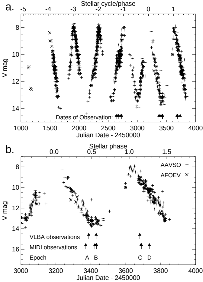
Fig. 1. Visual lightcurve of S Ori as a function of Julian Date and stellar cycle/phase. Data are from the AAVSO (Henden et al. 2006) and AFOEV (CDS) databases. We adopt a period of P = 430 days and JD of last maximum brightness T_0 = 2453190 . The arrows indicate the dates of our VLTI and VLBA observations. a) The most recent 5–6 cycles illustrating the correspondence of the data with our adopted P and T_0 values. The indicated dates of observations are the epochs from BW05 (JD between 2600 and 2800) and the epochs of the present paper (JD between 3300 and 3800). b) Enlarged view covering our VLTI/MIDI and VLBA observations presented in this paper. The dates of observations are combined into 4 epochs A, B, C, D.
