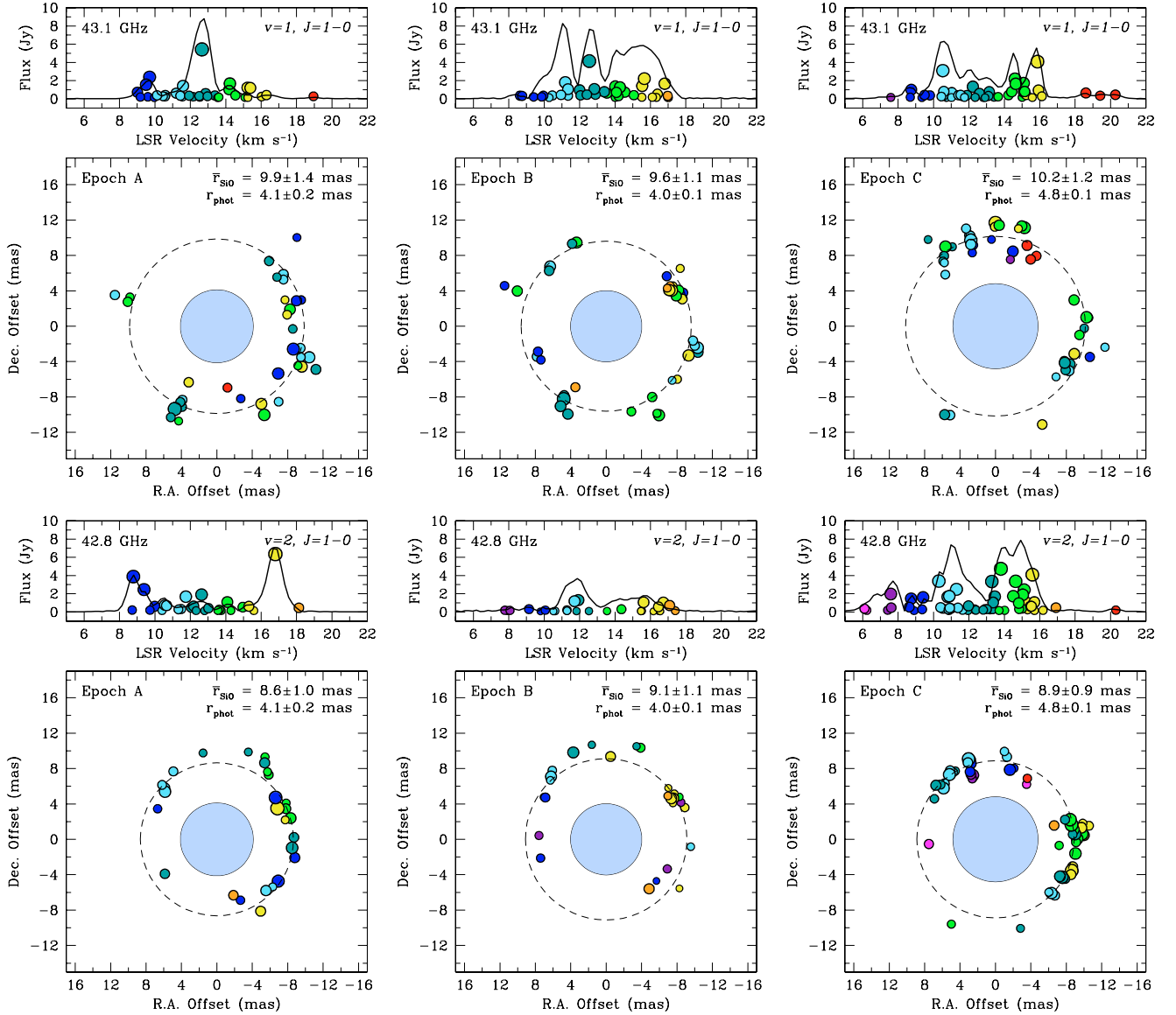
Fig. 8. LOS velocity structure of the (top) v = 1, J = 1-0 (43.1 GHz) and (bottom) v = 2, J = 1-0 (42.8 GHz) SiO maser emission toward S Ori. The epochs of observations are from left to right Epoch A ( \Phi_{\text{vis}} = 0.46 ), Epoch B ( \Phi_{\text{vis}} = 0.56 ), and Epoch C ( \Phi_{\text{vis}} = 1.14 ). The top sub-panels of each epoch and transition show the spectra formed by plotting maser intensity versus velocity, color-coded in 1.7 \text{ km s}^{-1} velocity increments from redward to blueward. The solid lines in the top sub-panels represent the scalar-averaged cross-power spectra averaged over all of the VLBA antennas. The bottom (main) sub-panels plot the spatial and velocity distributions of the masers. The color of each point represents the corresponding velocity bin in the spectrum, and the size of each point is proportional to the logarithm of the flux density. Errors in the positions of the features are smaller than the data points. The dashed circles are based on the mean angular distances of the SiO masers from the centers of the distributions. The light blue filled circles in the centers illustrate for comparison the angular sizes of the continuum photosphere derived in Sect. 3.4. The true location of the star relative to the masers is unknown and here assumed to coincide with the center of the maser spot distribution. We use also panels (e) of Figs. 2–5, as well as Fig. 7, for a comparison of the SiO maser ring radii to the extension of the molecular atmosphere and the inner dust shell boundary.
