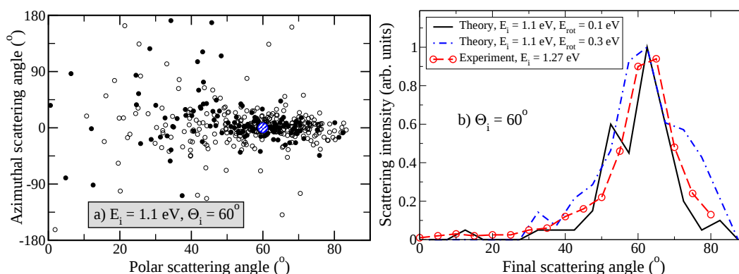
Figure 10: Angular distribution of \text{O}_2 scattered from Pt(111) with an angle of incidence of 60^\circ . a) Calculated angular distribution (surface temperature T_s = 300 K) for an initial rotational energy of 0.1 eV (filled circles) and 0.3 eV (open circles). b) Comparison of the measured and the calculated angular distribution in in-plane scattering for an angle of incidence of 60^\circ . The initial kinetic energy in the experiment was 1.27 eV [85] while the TBMD simulations have been performed for an initial energy of 1.1 eV. Theoretical results are shown for both an initial rotational energy of 0.1 eV and 0.3 eV.
