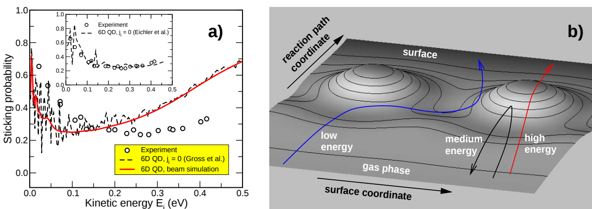
Figure 7: Dissociative adsorption of H_2/Pd(100) . a) Sticking probability of H_2/Pd(100) as a function of the initial kinetic energy. Circles: experiment [51], dashed and solid line: theory according to H_2 initially in the ground state and with a thermal distribution appropriate for a molecular beam [49]. The inset shows the theoretical results using an improved ab initio potential energy surface [52]. b) Illustration of the steering effect.
