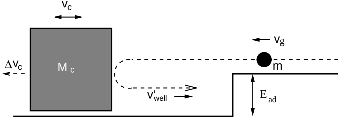
Figure 4: Hard cube model. a) Schematic illustration of the model. An atom or molecule with mass m is impinging in an attractive potential with well depth E_{ad} on a surface modeled by a cube of effective mass M_c . The surface cube is moving with a velocity v_c given by a Maxwellian distribution. b) Trapping probability as a function of the kinetic energy evaluated according to the hard cube model Eq. (26) for different adsorption energies E_{ad} , mass ratios \mu = m/M_c and surface temperatures T_s .
