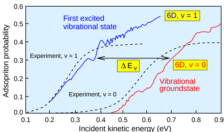
Figure 8: Dissociative adsorption probability of H_2 on Cu(100) as a function of the incident kinetic energy determined by six-dimensional quantum wave-packet calculations for molecules initially in the vibrational ground state and first excited state, respectively [61]. The calculations are compared to experimental results derived from an analysis of adsorption and desorption experiments [62].
