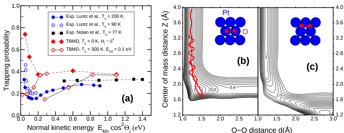
Figure 9: \text{O}_2 adsorption on Pt(111). a) Trapping probability of \text{O}_2/\text{Pt}(111) as a function of the normal component of the kinetic energy. Results of molecular beam experiments for surface temperatures of 90 K and 200 K (Luntz et al. [78]) and 77 K (Nolan et al. [79]) are compared to tight-binding molecular dynamics simulations for the surface initially at rest ( T_s = 0 K). b and c) Elbow plots of the PES of the dissociation of \text{O}_2/\text{Pt}(111) determined by the ab initio derived tight-binding Hamiltonian [76, 83]. The configurations of the remaining \text{O}_2 degrees of freedom are illustrated in the insets. The contour spacing is 0.2 eV per \text{O}_2 molecule. In (b) a trajectory of an \text{O}_2 molecule with an initial kinetic energy of 0.6 eV scattered at Pt(111) is also plotted.
