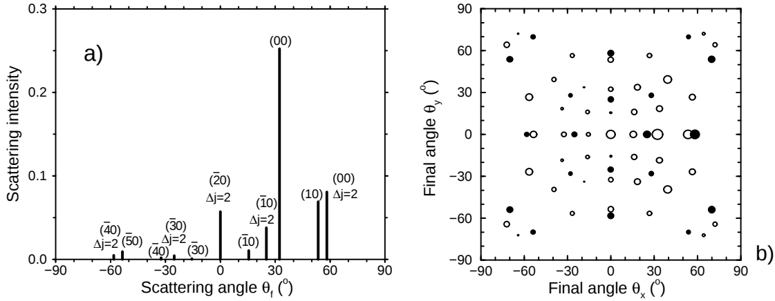
Figure 3: Diffraction spectrum of \text{H}_2 scattered at \text{Pd}(100) for a kinetic energy of 76 meV at an incidence angle of 32^\circ along the [10] direction of the square surface lattice, obtained by six-dimensional quantum coupled channel calculations. a) In-plane diffraction spectrum where all peaks have been labeled according to the transition. b) In-plane and out-of-plane diffraction peaks. The open and filled circles correspond to the rotationally elastic and rotationally inelastic scattering, respectively, with the radius of the circles being proportional to the logarithm of the scattering intensity (after [26]).
