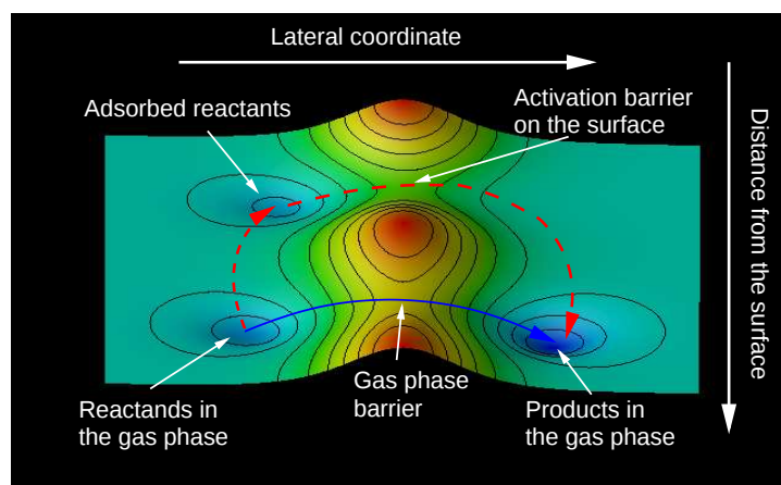
Figure 1: Schematic illustration of the role of a catalyst using a two-dimensional representation of the potential energy surface. A catalyst provides a detour in the multi-dimensional PES with lower activation barriers
