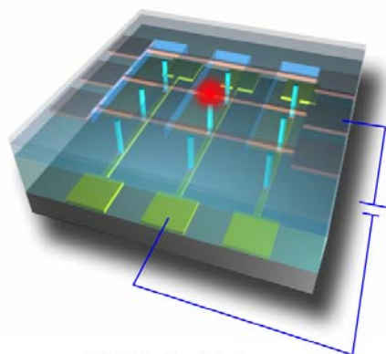
Field-Emitter Display
