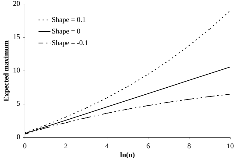
Figure 5.2: The effect of the shape parameter ( \xi ) on the expected maximum of n independent draws from a GEV distribution.
