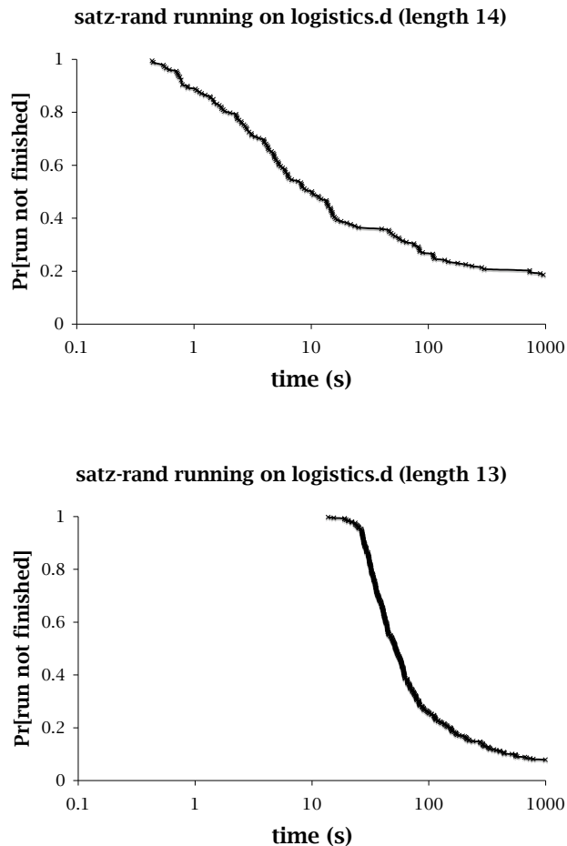
Figure 3.1: Run length distribution of satz-rand on two formulae created by SATPLAN in solving the logistics planning instance logistics.d . Each curve was estimated using 150 independent runs, and run lengths were capped at 1000 seconds.
