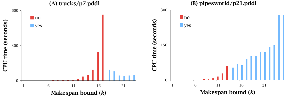
Figure 4.3: Behavior of the SAT solver siege running on formulae generated by SATPLAN to solve (A) instance p7 from the trucks domain and (B) instance p21 from the pipesworld domain of the 2006 International Planning Competition.
