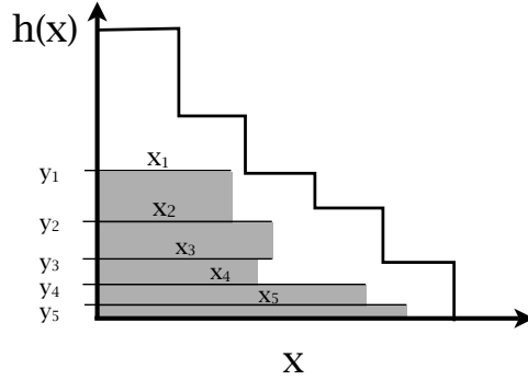
Figure 2.1: An illustration of the inequality \int_{x=0}^{\infty} h(x) dx \geq \sum_{j \geq 1} x_j (y_j - y_{j+1}) . The left hand side is the area under the curve, whereas the right hand side is the sum of the areas of the shaded rectangles.
