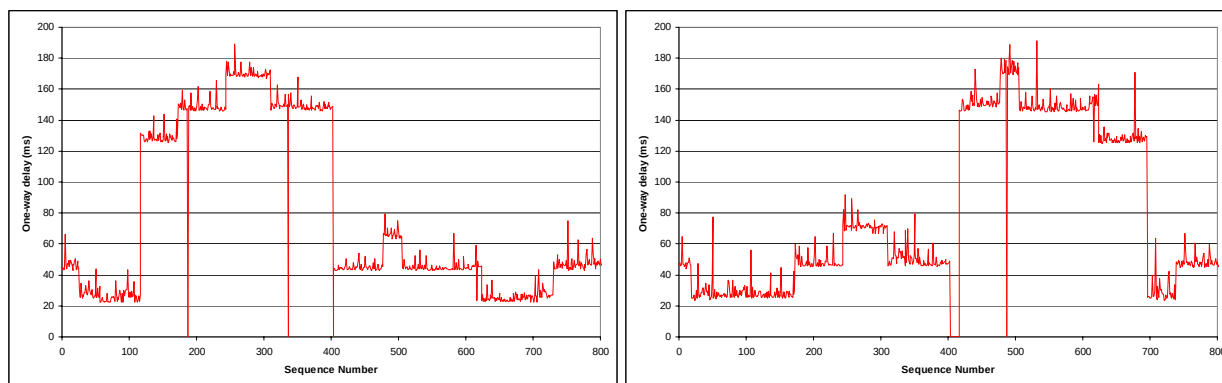
Figure 3-8: Egress traffic latency –from Mobile to Host 1 (left) and to Host 2 (right).
