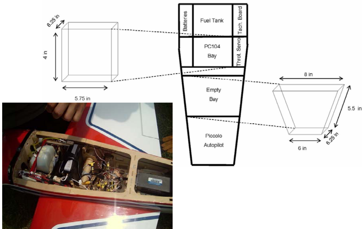
Figure 5-1: UIUC UAV.
