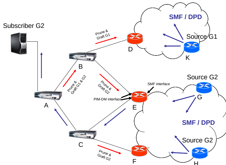
Figure 2-9: Multicast gateway concept of operations.
