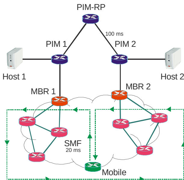
Figure 3-6: Experimental topology depicting MANET Border Routers (MBR) interacting with Simplified Multicast Forwarding (SMF) mobile nodes and PIM-Sparse Mode routers.
