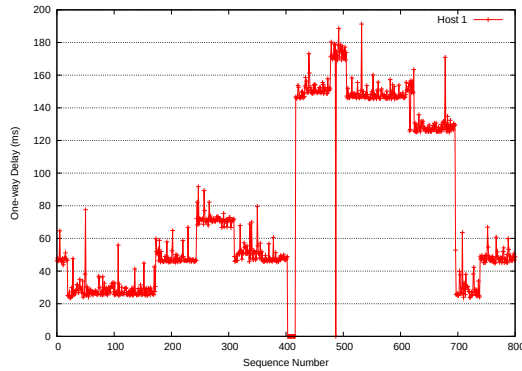
Fig. 12. Egress to Host 1: Latency.
