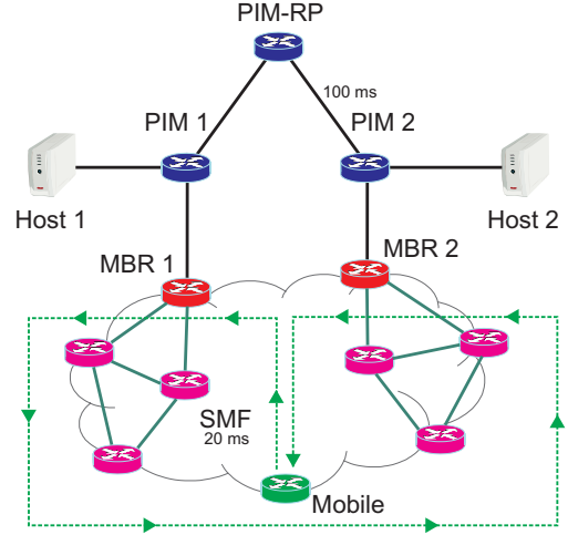
Fig. 10. Experiment topology
