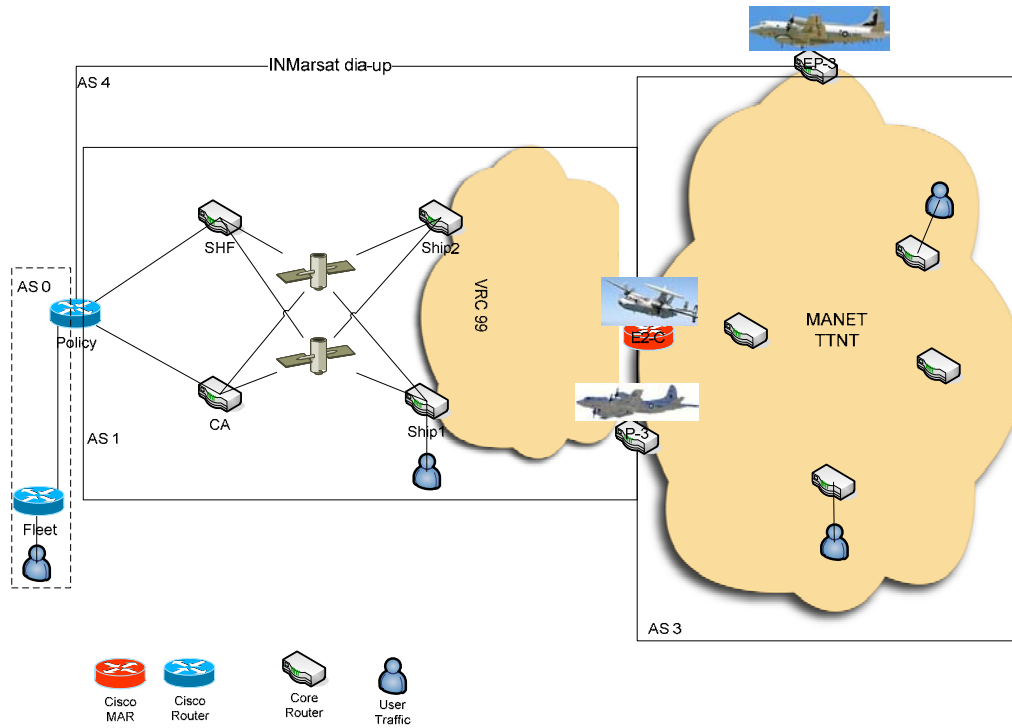
Figure 3-2: Simulation/emulation scenario of ADNS shore, ships and airborne elements for studying routing integration and route redistribution.
