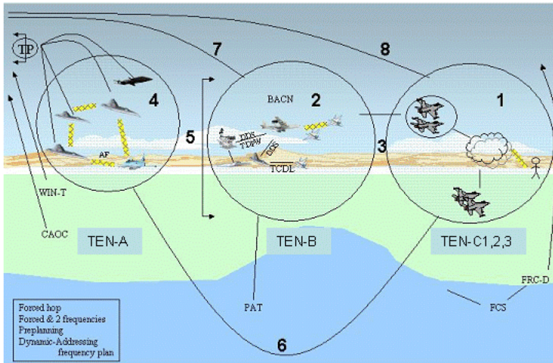
Figure 2-2. TEN-C Spiral 1-3 [from GIG JTEN]
