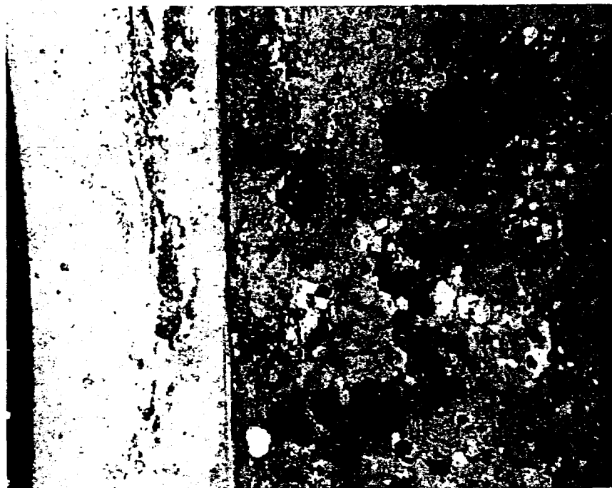
FIGURE 4. SECTION OF 90:10 COPPER-NICKEL PIPING FROM THE AFT MASKER COOLING DISCHARGE WITH DEEP PITTING CLOSE TO THE FLANGE
