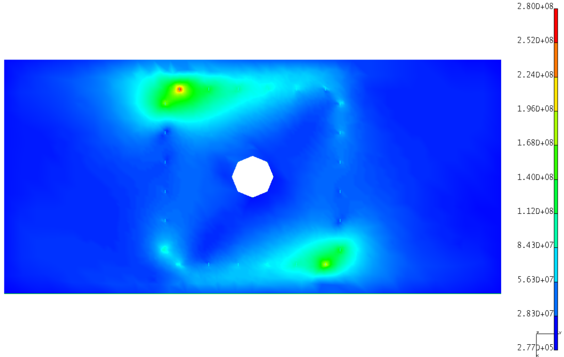
Figure 39: D-advanced structure with square bolt pattern, 15mm shell, 24 bolts, 72 elements
