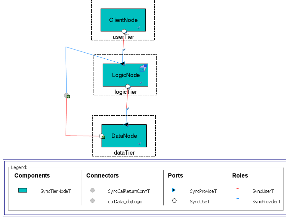
Figure 11: Conformance results between the CourSys as-designed and as-built architecture.
