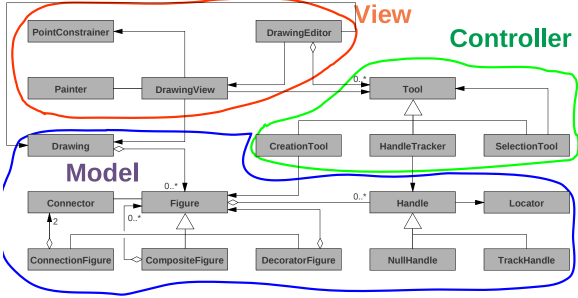
Figure 15: JHotDraw class diagram (Source: [61]).
