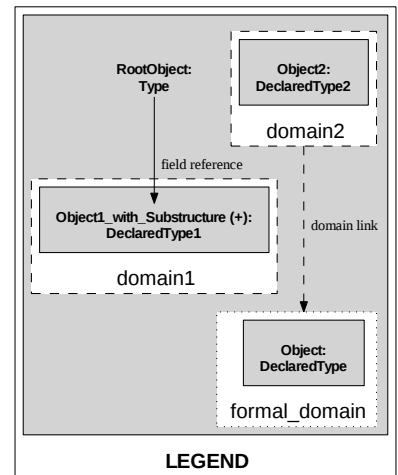
(c) Ownership Object Graph legend.
