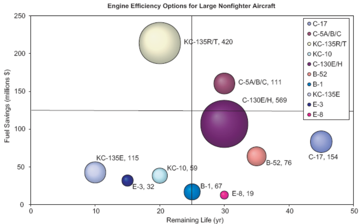
Figure 9 Engine Efficiency Options for Large Nonfighter Aircraft. Copyright © National Academy of Sciences. Permission is granted for this material to be shared for noncommercial, educational purposes, provided that this notice appears on the reproduced materials, http://www.nap.edu/catalog.php?record_id=11837 .
