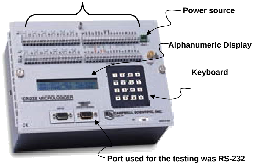
Figure 1. The CR23X Micrologger.
