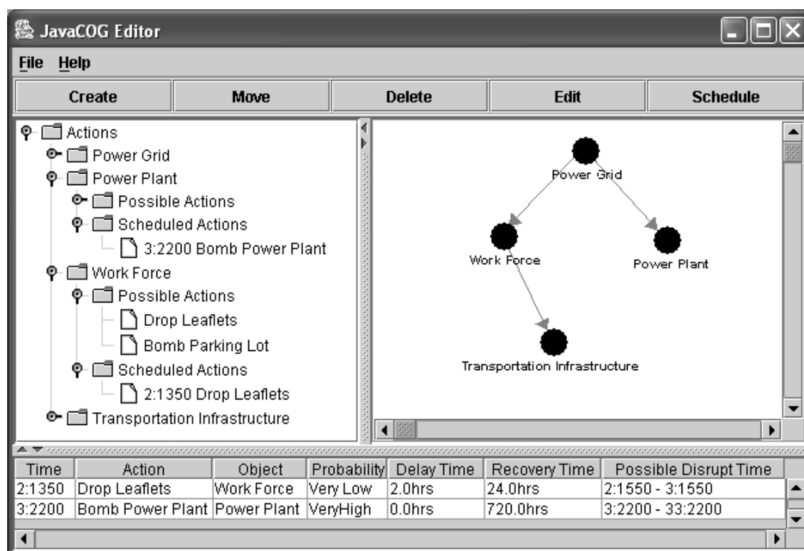
Figure 2. Example of JavaCOG
