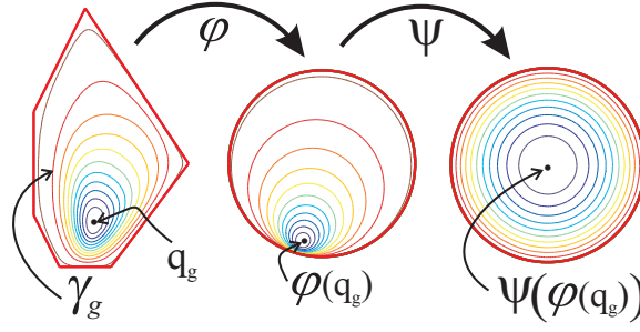
Figure 4.3: Equipotential contours for a convergent potential function found by mapping the goal cell to a unit ball centered at the goal, and letting \gamma_g = \frac{1}{2} \|\psi \circ \phi\|^2 .
