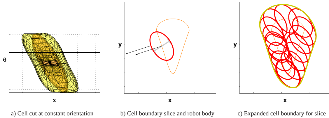
Figure C.6: The calculation of the extended surface is based on a planar Minkowski sum. a) Consider a slice of the cell at constant orientation. b) The robot body is placed along the boundary of the cell for this constant orientation. The corresponding point on the expanded surface is found by matching normals for the planar cell boundary and the robot body. c) The boundary of the extended cell is calculated.
