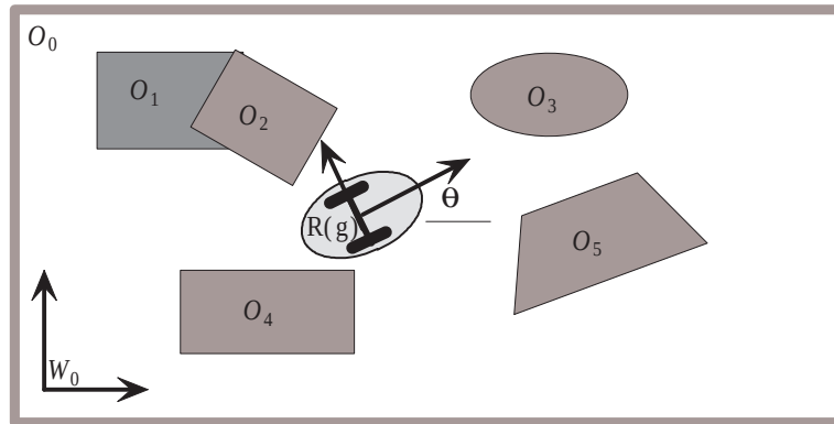
Figure A.1: Representation of planar workspace with five obstacles and robot. The workspace frame is denoted W_0 ; the body pose relative to W_0 is denoted g = \{x, y, \theta\} . The body occupies R(g) \subset \mathcal{W} . The workspace boundary is denoted as O_0 .
