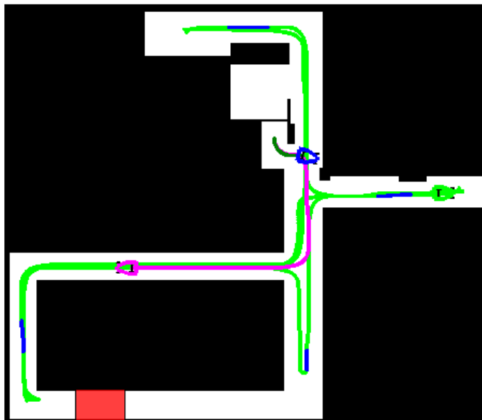
Figure 6.22: As new information becomes available, such as the obstacle in the lower corridor, the automaton synthesis formulates a different automaton based on changes to the prepared graph. The new automaton preserves the correct behavior.
