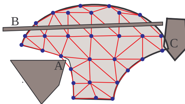
Figure C.7: Collision tests on the approximation of R(\Xi_i) using overlapping facets. The light gray region denotes a representation of R(\Xi_i) . The grid and facets shows the approximation based on the projection of expanded cell surface mesh. The dark gray obstacle on the left labeled ‘A’ does not intersect R(\Xi_i) ; however, the approach classifies the cell as unsafe based on the facet intersection near point ‘A’. Obstacle ‘B’ intersects R(\Xi_i) , but the approximate tests misses the fact as no vertices in ‘B’ are contained in a facet, and no facet vertices are contained in ‘B’. The obstacle labeled ‘C’ on the right does intersect R(\Xi_i) , but the approximation misses this collision.
