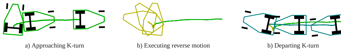
Figure 6.13: Plot of data from actual robot experiment as the robot executes a K-turn in the upper hallway. The K-turn is automatically induced by the composition of policies based on simple arcs and straight path segments.
