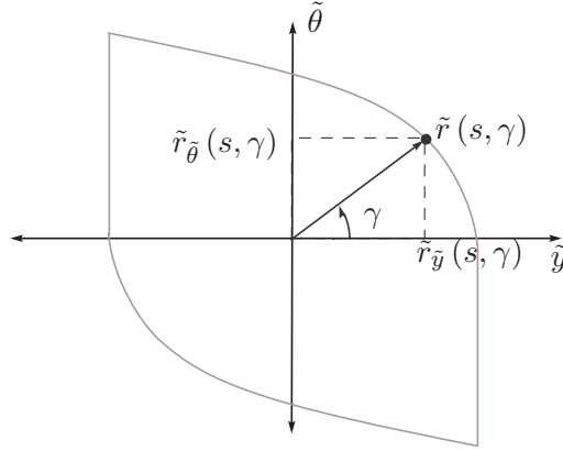
Figure D.12: PF cell boundary definitions for defining parameterized representation.
