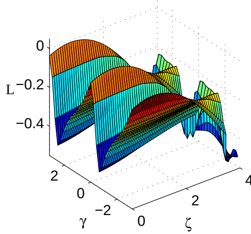
Figure E.3: Constraint surface for L(\zeta, \gamma) from (E.4).
