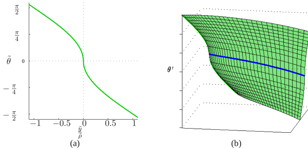
Figure D.3: PF control surface: a) Sliding control surface in the local \mathcal{F}_{\tilde{y}}-\mathcal{F}_{\tilde{\theta}} plane defined by (D.1). b) Sliding control surface in body pose space formed by extruding the local curve along the \hat{g}(s) curve.
