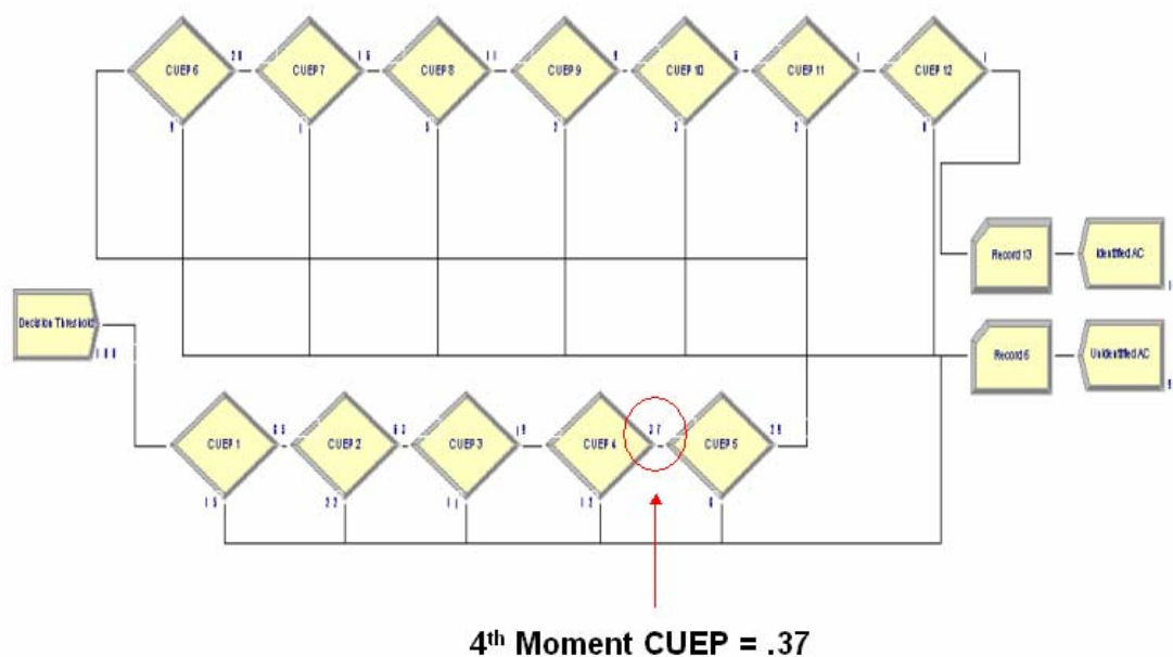
Figure 5. Alternative Model Simulation
