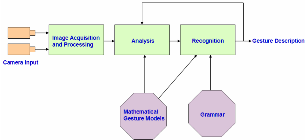
Figure 1 Gesture Interpretation System
