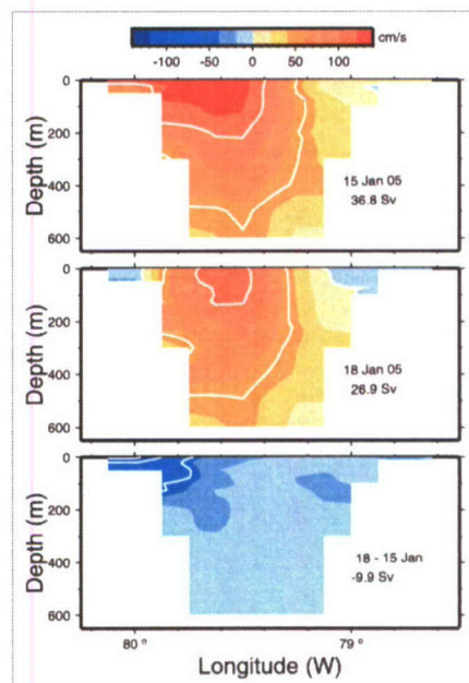
Fig. 3. Transects (27°N) of along-channel velocity from G-NCOM. (top) At local maximum transport (15 January 2005). (middle) At local minimum transport (18 January 2005). (bottom) The 18–15 January difference field. Plotted from the z-level analysis grid provided by NAVOCEANO.
