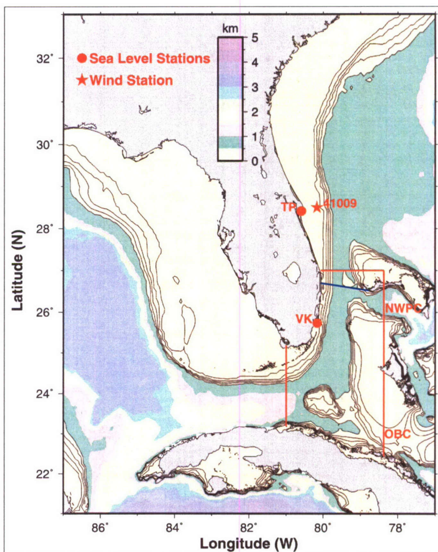
Fig. 1. Straits of Florida locator map. Blue line indicates cable, red lines indicate NCOM control volume. OBC is Old Bahamas Channel, NWPC is the Northwest Providence Channel, meteorological buoy (NDBC 41009), and coastal sea level stations are: TP, Trident Pier; VK, Virginia Key.
