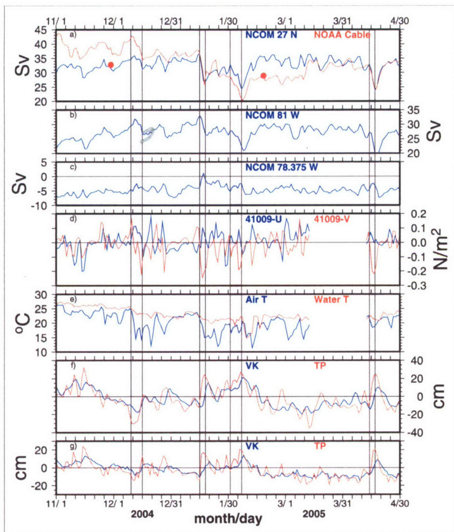
Fig. 2. Transport and related daily time series, 1 November 2004 to 30 April 2005. Shaded time periods are discussed in the article. (a) Cable and G-NCOM transport (27°N) (red circles are dropsonde section transports). (b) G-NCOM transport (81°W). (c) G-NCOM transport (78.375°W). (d) Wind stress components (NDBC 41009). (e) Surface atmospheric and oceanic temperature (NDBC 41009). (f) Subtidal observed coastal sea level (TP, Trident Pier; VK, Virginia Key). (g) Subtidal G-NCOM coastal sea level (interpolated to TP and VK sites). NDBC buoy 41009 has a data gap from 14 March to 11 April.
