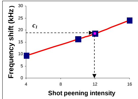
FIGURE 8. Using the y-intercept c_1 from a fitted curve and a correlation curve from the experimental data, the interpolation gives the estimated shot peening intensity of materials under test.
