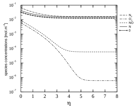
Figure 41: Species concentrations in the boundary layer for T_w = 1500K using the phenomenological model. The boundary layer is assumed to be frozen.
