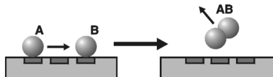
Figure 27: Langmuir-Hinshelwood (L-H) type recombination process
