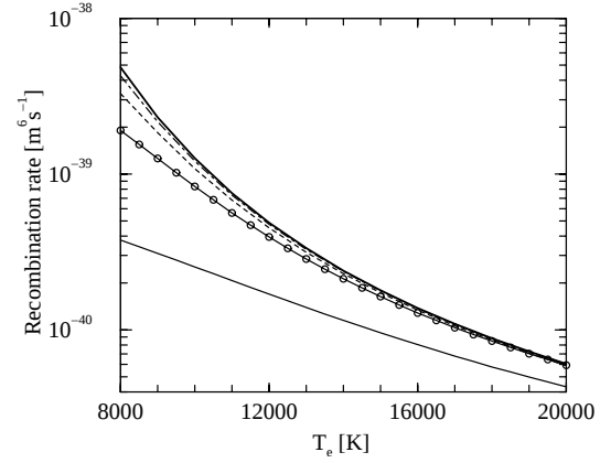
Figure 6: Recombination rate in optically thick cases as a function of T_e . Thick solid line: our 40 level model. Thin solid line: 9 levels. Solid line with open circles: 15 levels. Dashed line: 20 levels. Dot-dashed line: 30 levels.
