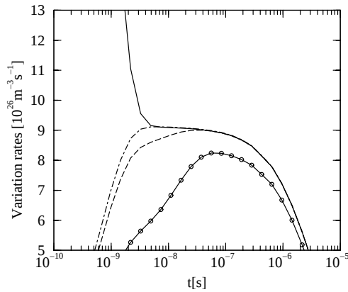
Figure 3: For the same initial recombining condition as in Figure 2. Solid line: |n_e| . Solid line with open circles: \dot{N}_1 . Dashed line: \dot{N}_1 + \dot{N}_2 . Dot-dashed line: \dot{N}_1 + \dot{N}_2 + \dot{N}_3 .
