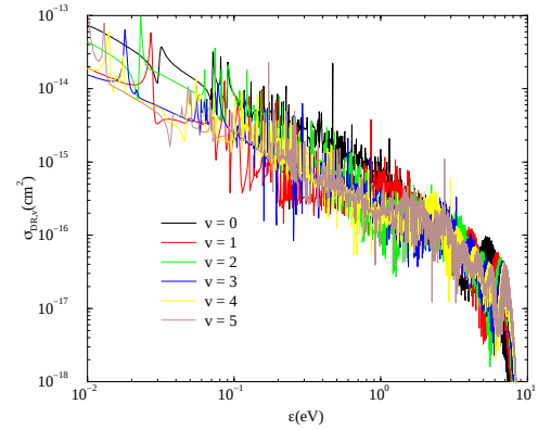
Figure 14: Cross section \sigma_{DR}(\epsilon, v) for dissociative recombination of NO^+ with electron for different vibrational excitation of the ion ( 0 \leq v \leq 5 ).
