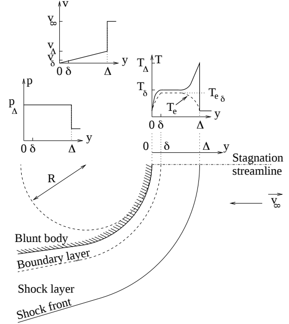
Figure 16: Considered situations of re-entry displaying the pressure, velocity and temperatures profiles along the stagnation streamline.
