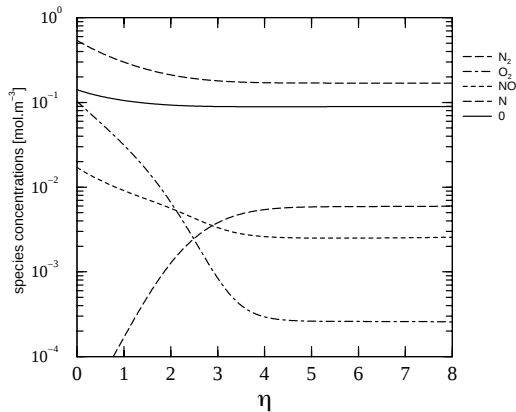
Figure 33: Species concentrations in the boundary layer for T_w = 1500K using the phenomenological model. The kinetic scheme of Dunn and Kang is used.
