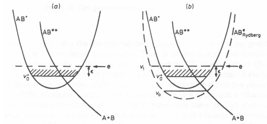
Figure 13: Schematic view of the two channels allowing the dissociative recombination of a molecular ion AB with electron. Left: the direct process, right: the indirect process. The electron energy is \epsilon . AB^{**} is a dissociative potential curve of the molecule AB .
