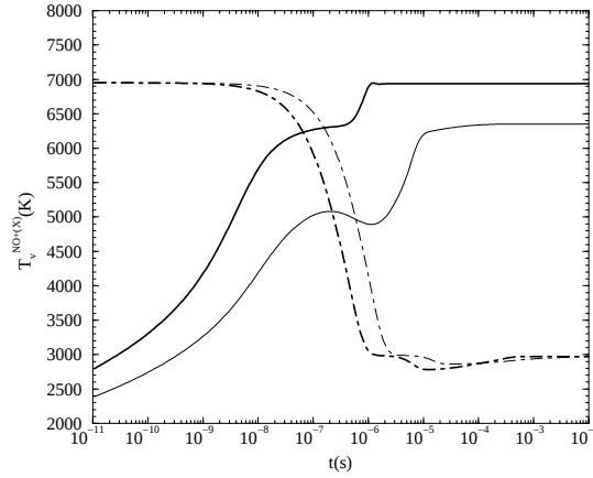
Figure 19: Time evolution of the vibrational temperature of NO^+(X^1\Sigma^+) in the case of Fig.17, the gas having crossed the shock front and whose temperatures are such that T_e = T_A = 7000\text{ K} (thick line) or 5000\text{ K} = T_e < T_A = 7000\text{ K} (thin line). The thin dot-dashed line refers to the typical recombination inside the boundary layer with p = 2\text{ kPa} from T_e = T_A = 7000\text{ K} to T_e = T_A = 3000\text{ K} (see Fig.20 and 21) and the thick dot-dashed line refers to the same situation but with p = 10\text{ kPa} (see Fig.22 and 23).
