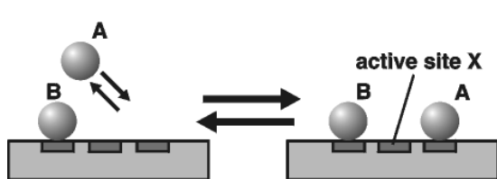
Figure 25: atom adsorption/desorption
