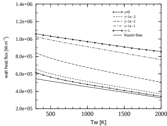
Figure 29: Wall heat flux as a function of the wall temperature for different values of the average \gamma coefficient. The kinetic scheme of Dunn and Kang is used.
