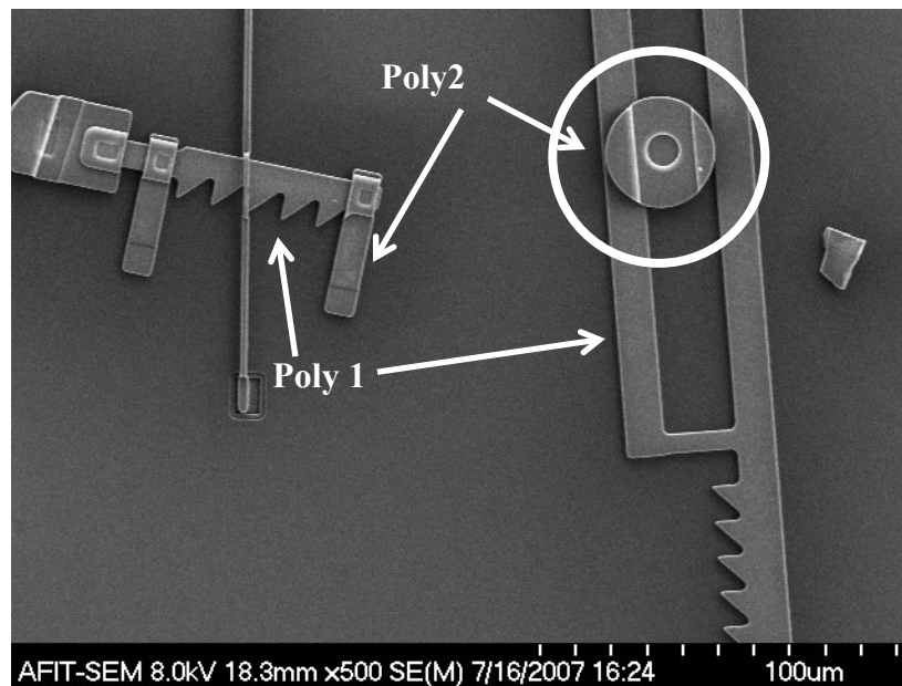
Figure 45: SEM photo of pawl arm requiring rotation with circled pin
