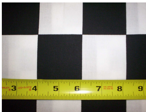
Figure 18: Calibration Checkerboard Dimensions. Squares are 53.975 mm x 53.975 mm on each side.
