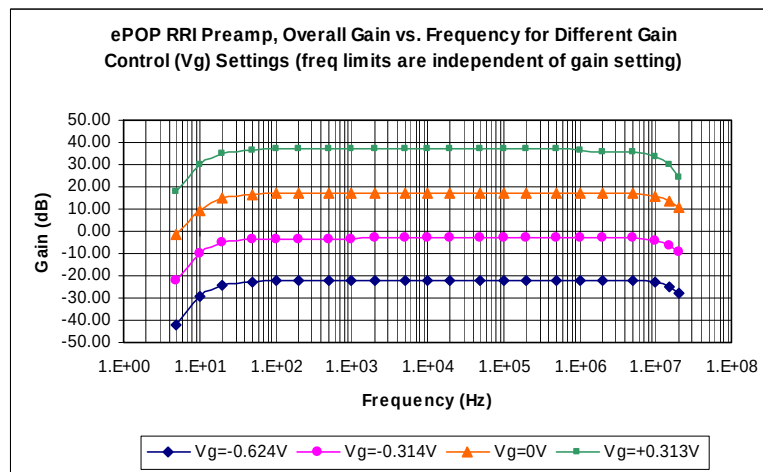
Figure 5: Preampifier Bandwidth.
