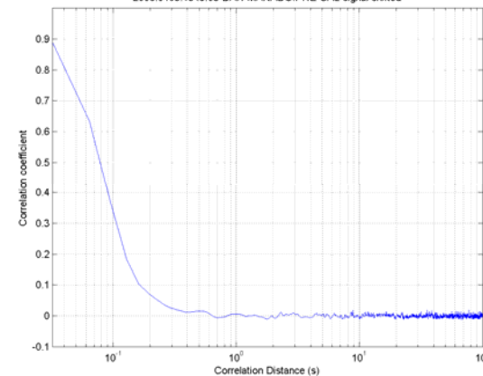
AUTOCORRELATION FUNCTION OF (LINEAR) FADING POWER 2006.0405.1349.05-DAR-MANADO.PRE-CAL-signal-shifted
