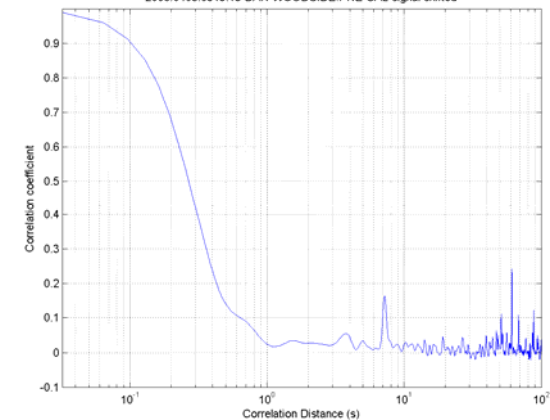
AUTOCORRELATION FUNCTION OF (LINEAR) FADING POWER 2006.0403.0919.15-DAR-WOODSIDE.PRE-CAL-signal-shifted
