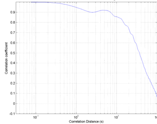
AUTOCORRELATION FUNCTION OF (LINEAR) FADING POWER 2006.0405.1349.05-DAR-MANADO.PRE-CAL-signal-shifted
