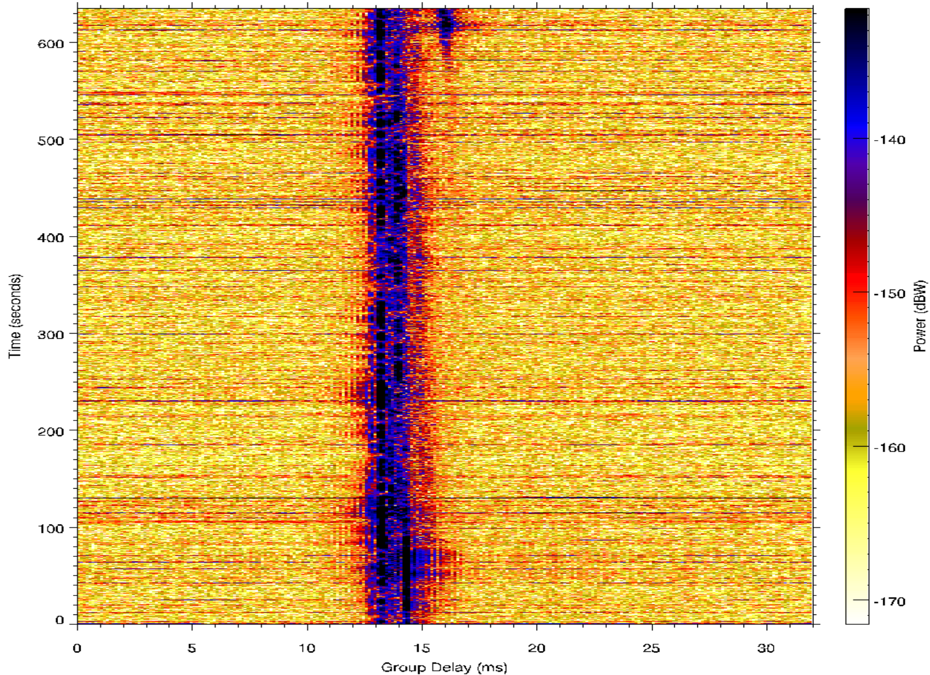
Cocos Is. --> Darwin Rx 2006 D:096 6-Apr 07:15:00 Channel Impulse Response
