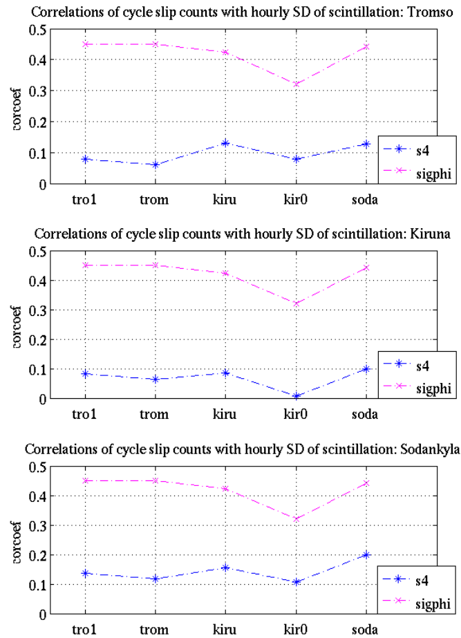
Figure 4: Correlations between the scintillation measured by the Novatel receivers and number of cycle-slips in the IGS receivers.
