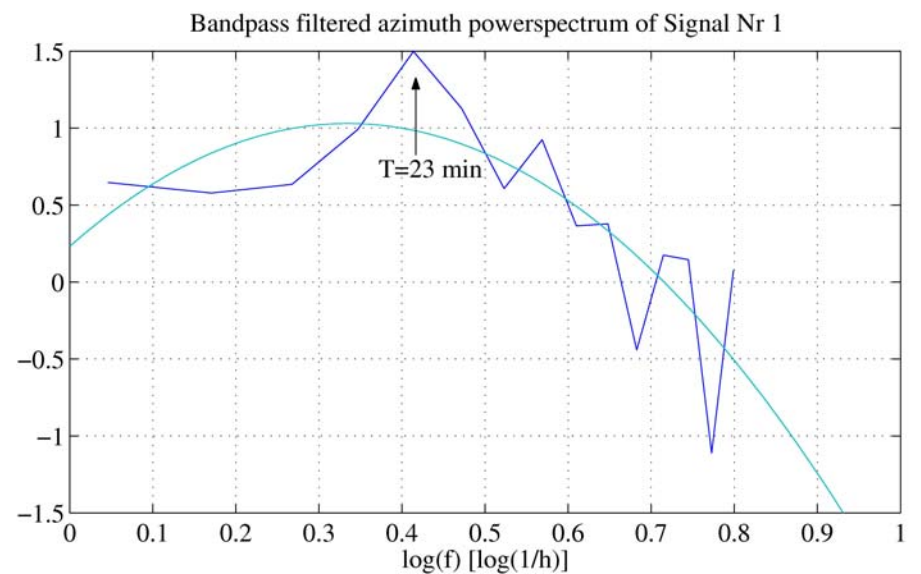
Associated log power spectrum to the temporal profile
