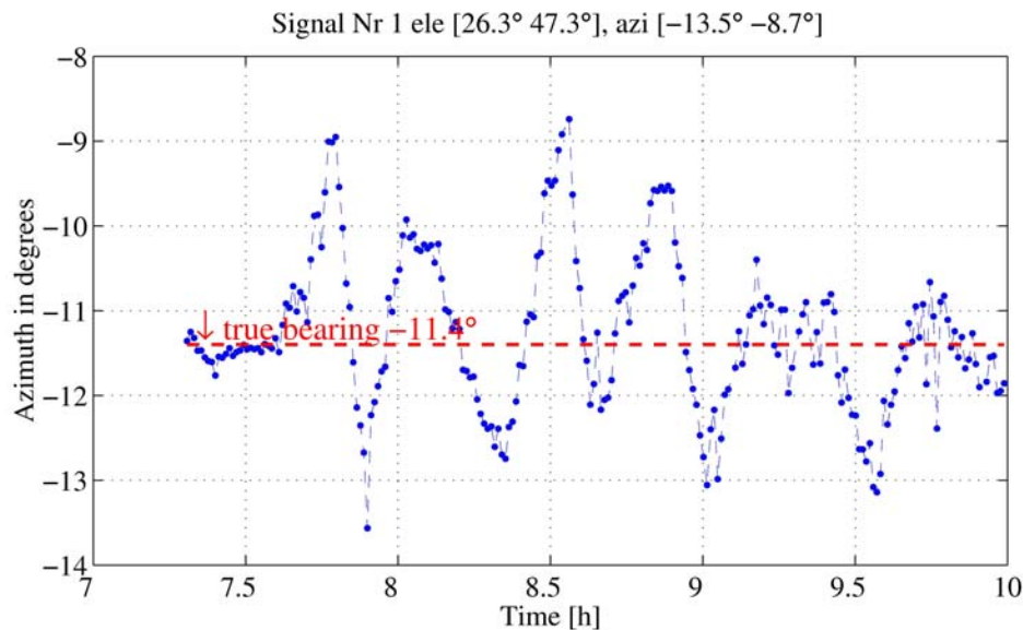
Signature of a traveling wave packet on the forenoon of 24.4.02
