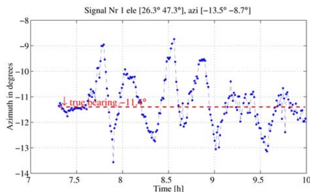
Figure 6: Signature of a traveling wave packet on the forenoon of 24.4.02
